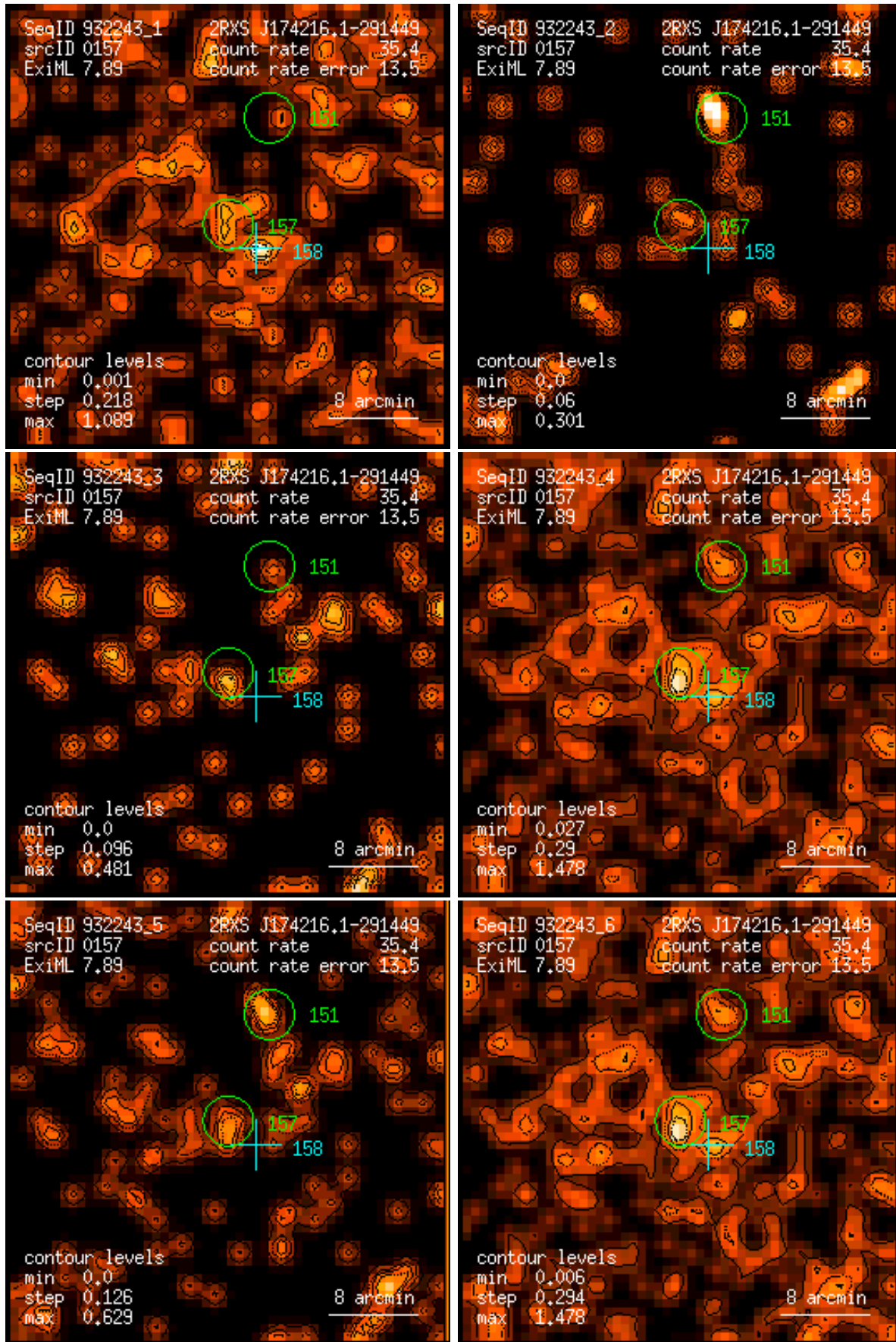
Figure 157: RASS 932243: detection 0157: band rate images, Gaussian filter: (1) PSPC channels 11 – 41, (2) 52 – 90, (3) 91 – 201, (4) 11 – 235, (5) 52 – 201, (6) 11 – 201. Broad band rates in counts/ks. Band rate contour levels in counts/ks/arcmin 2 .
