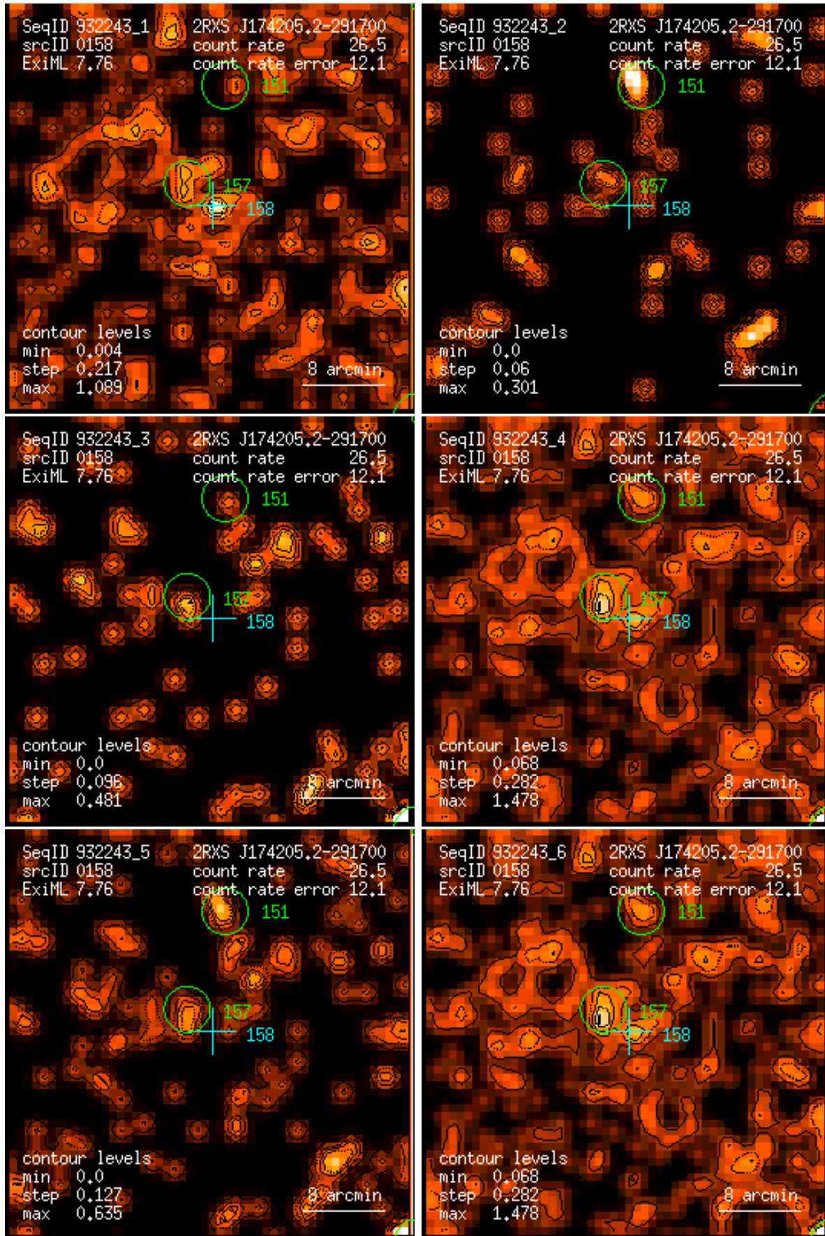
Figure 158: RASS 932243: detection 0158: band rate images, Gaussian filter: (1) PSPC channels 11 – 41, (2) 52 – 90, (3) 91 – 201, (4) 11 – 235, (5) 52 – 201, (6) 11 – 201. Broad band rates in counts/ks. Band rate contour levels in counts/ks/arcmin 2 .
