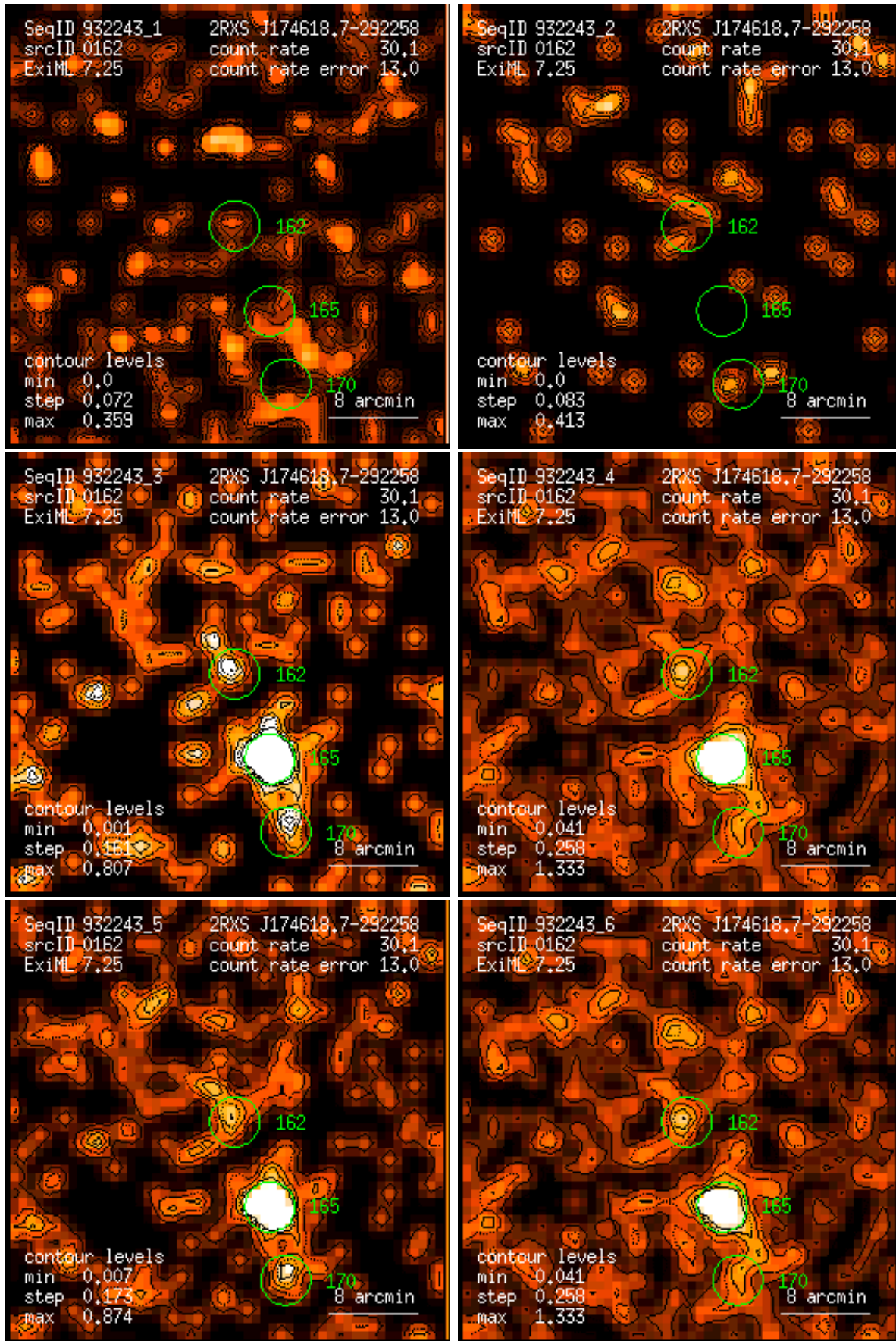
Figure 162: RASS 932243: detection 0162: band rate images, Gaussian filter: (1) PSPC channels 11 – 41, (2) 52 – 90, (3) 91 – 201, (4) 11 – 235, (5) 52 – 201, (6) 11 – 201. Broad band rates in counts/ks. Band rate contour levels in counts/ks/arcmin 2 .
