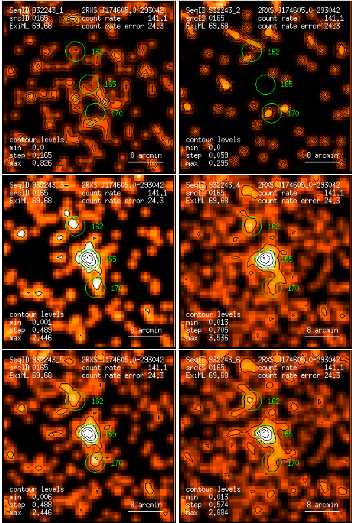
Figure 165: RASS 932243: detection 0165: band rate images, Gaussian filter: (1) PSPC channels 11 – 41, (2) 52 – 90, (3) 91 – 201, (4) 11 – 235, (5) 52 – 201, (6) 11 – 201. Broad band rates in counts/ks. Band rate contour levels in counts/ks/arcmin 2 .
