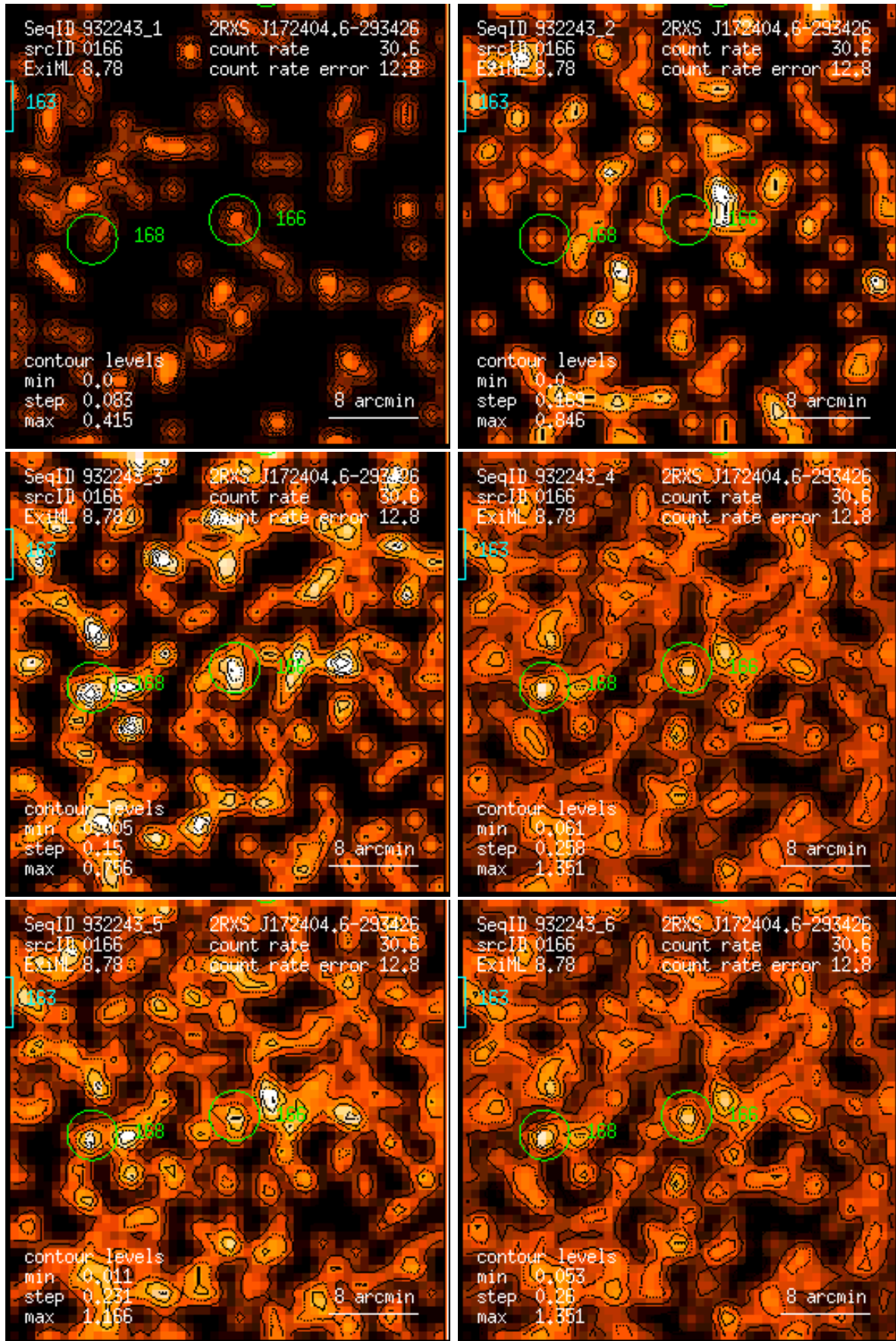
Figure 166: RASS 932243: detection 0166: band rate images, Gaussian filter: (1) PSPC channels 11 – 41, (2) 52 – 90, (3) 91 – 201, (4) 11 – 235, (5) 52 – 201, (6) 11 – 201. Broad band rates in counts/ks. Band rate contour levels in counts/ks/arcmin 2 .
