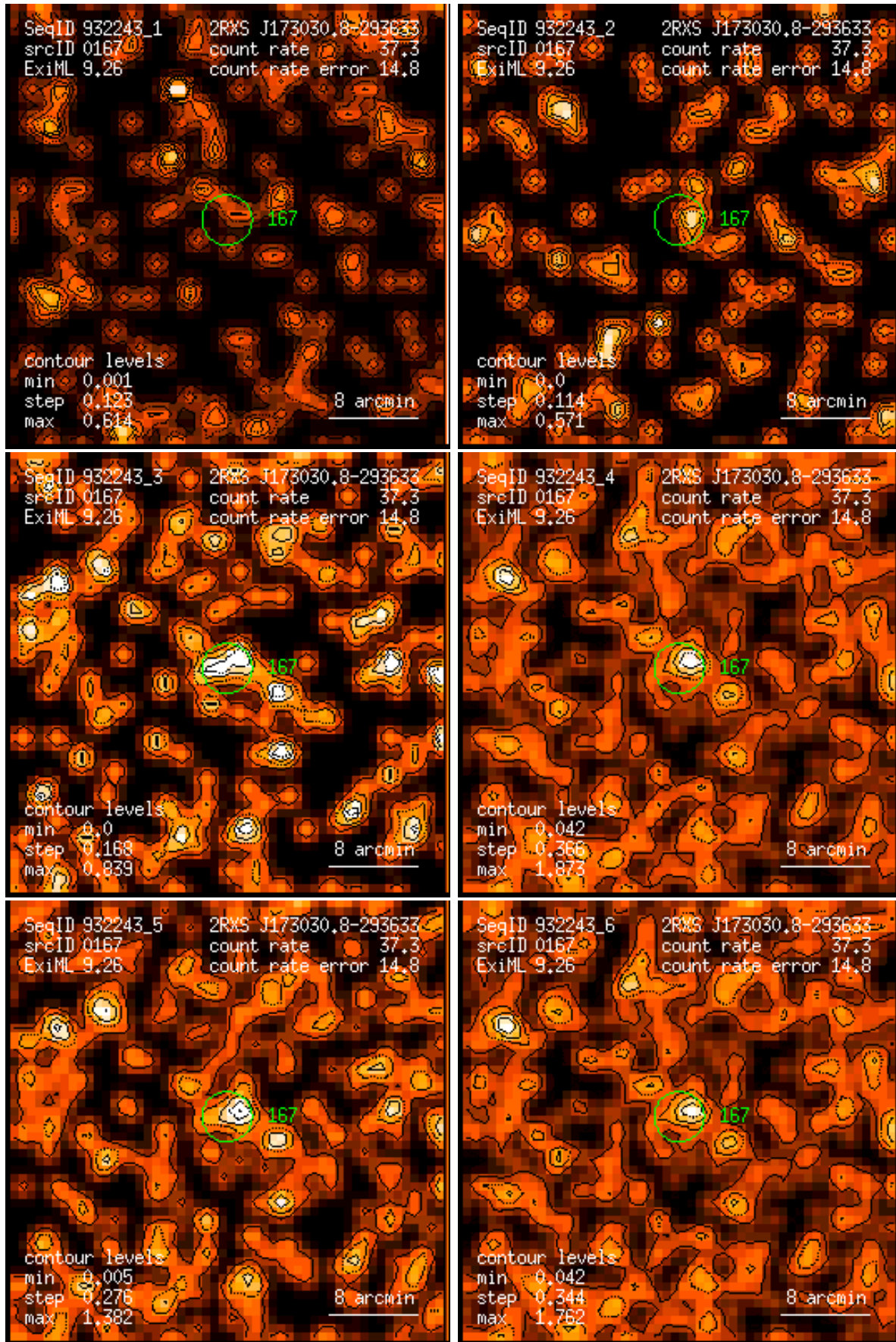
Figure 167: RASS 932243: detection 0167: band rate images, Gaussian filter: (1) PSPC channels 11 – 41, (2) 52 – 90, (3) 91 – 201, (4) 11 – 235, (5) 52 – 201, (6) 11 – 201. Broad band rates in counts/ks. Band rate contour levels in counts/ks/arcmin 2 .
