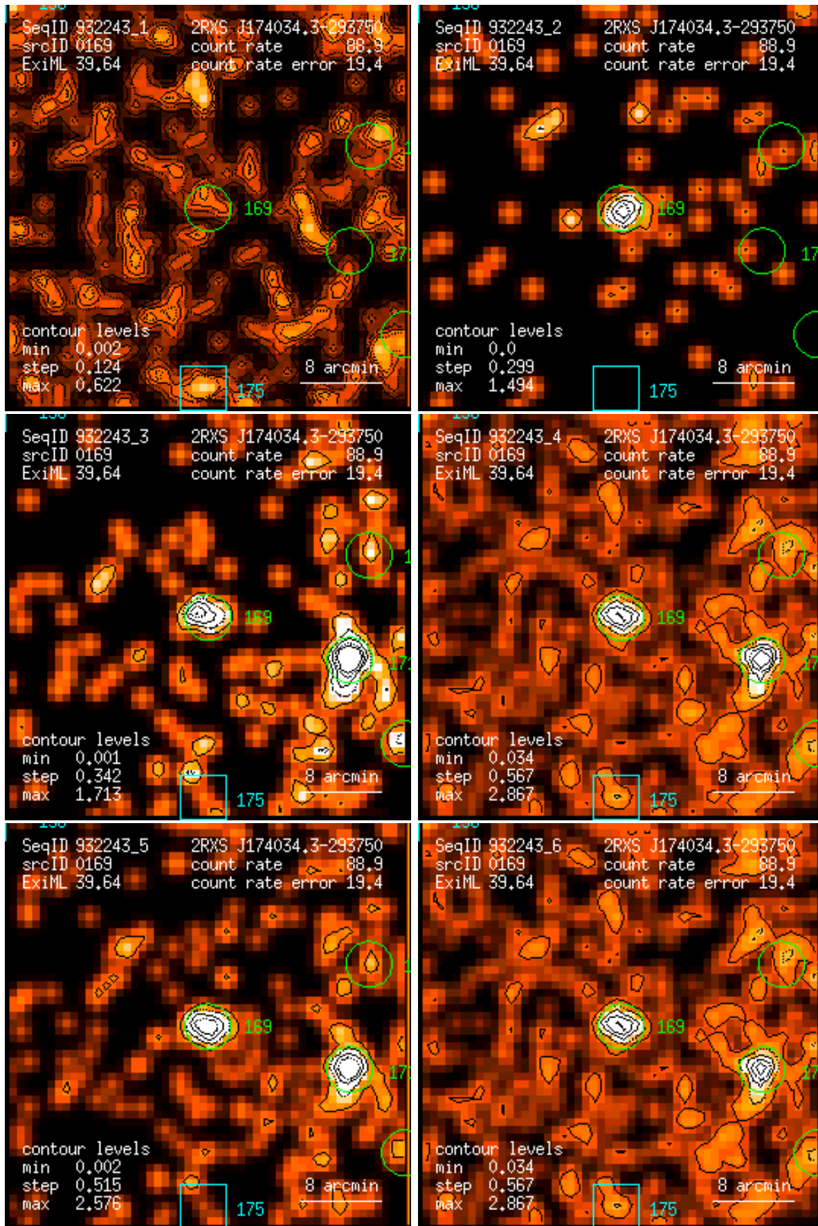
Figure 169: RASS 932243: detection 0169: band rate images, Gaussian filter: (1) PSPC channels 11 – 41, (2) 52 – 90, (3) 91 – 201, (4) 11 – 235, (5) 52 – 201, (6) 11 – 201. Broad band rates in counts/ks. Band rate contour levels in counts/ks/arcmin 2 .
