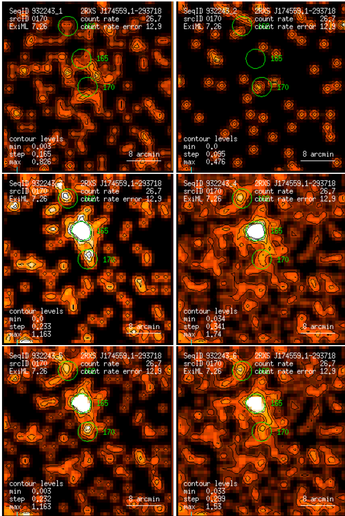
Figure 170: RASS 932243: detection 0170: band rate images, Gaussian filter: (1) PSPC channels 11 – 41, (2) 52 – 90, (3) 91 – 201, (4) 11 – 235, (5) 52 – 201, (6) 11 – 201. Broad band rates in counts/ks. Band rate contour levels in counts/ks/arcmin 2 .
