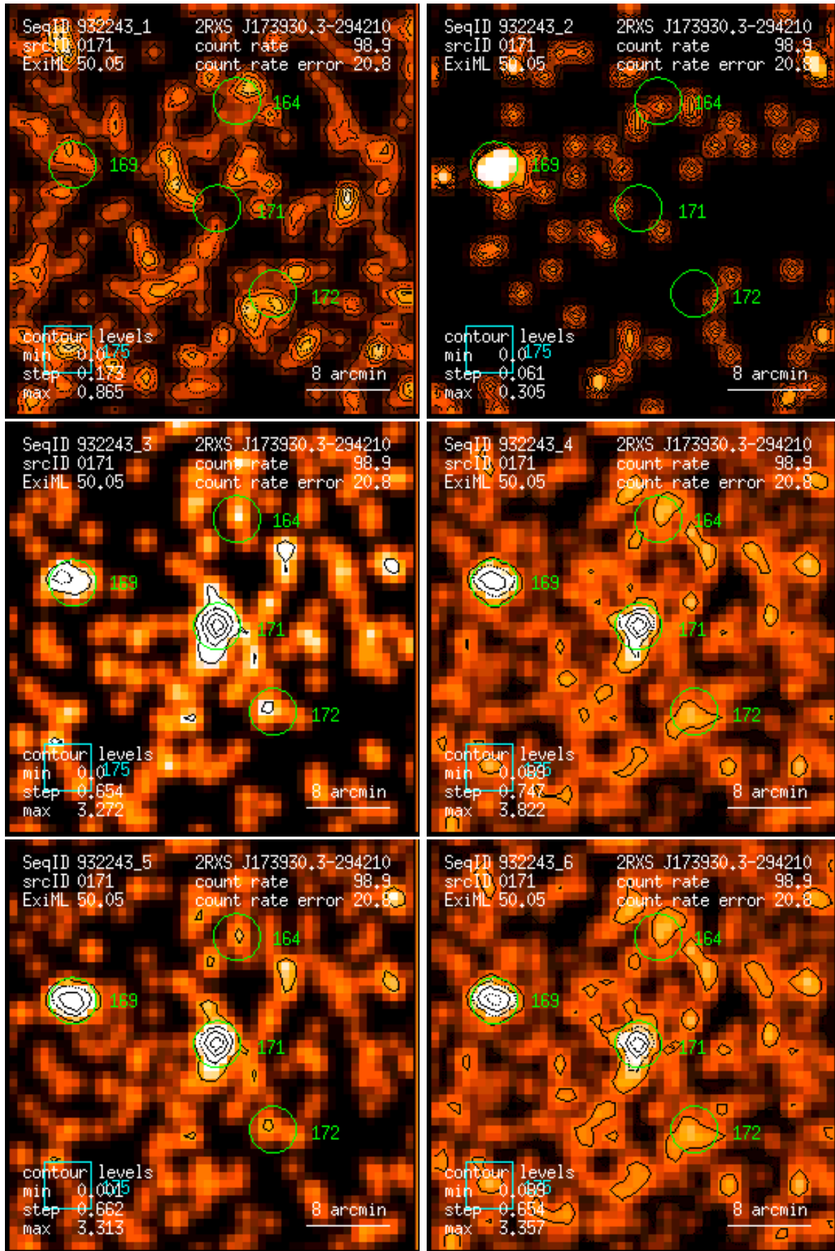
Figure 171: RASS 932243: detection 0171: band rate images, Gaussian filter: (1) PSPC channels 11 – 41, (2) 52 – 90, (3) 91 – 201, (4) 11 – 235, (5) 52 – 201, (6) 11 – 201. Broad band rates in counts/ks. Band rate contour levels in counts/ks/arcmin 2 .
