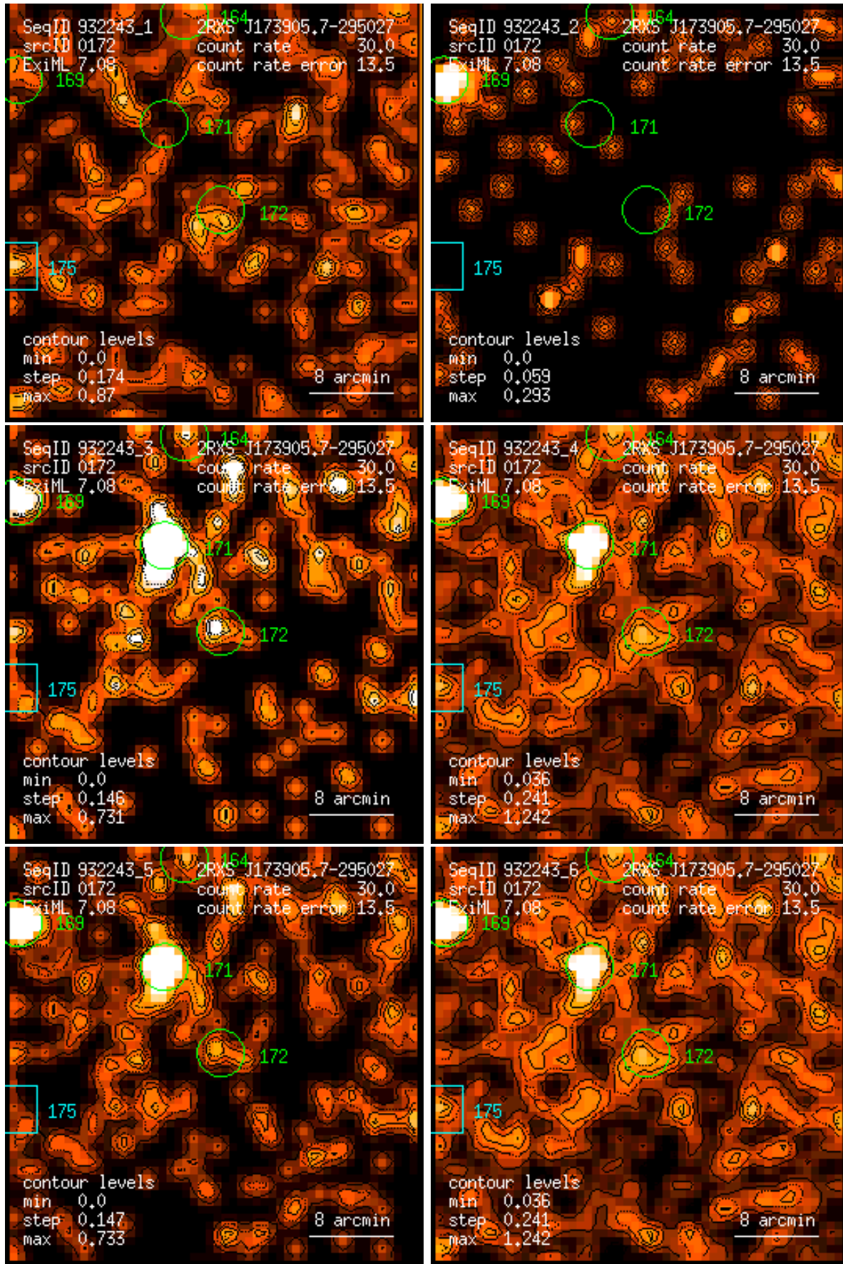
Figure 172: RASS 932243: detection 0172: band rate images, Gaussian filter: (1) PSPC channels 11 – 41, (2) 52 – 90, (3) 91 – 201, (4) 11 – 235, (5) 52 – 201, (6) 11 – 201. Broad band rates in counts/ks. Band rate contour levels in counts/ks/arcmin 2 .
