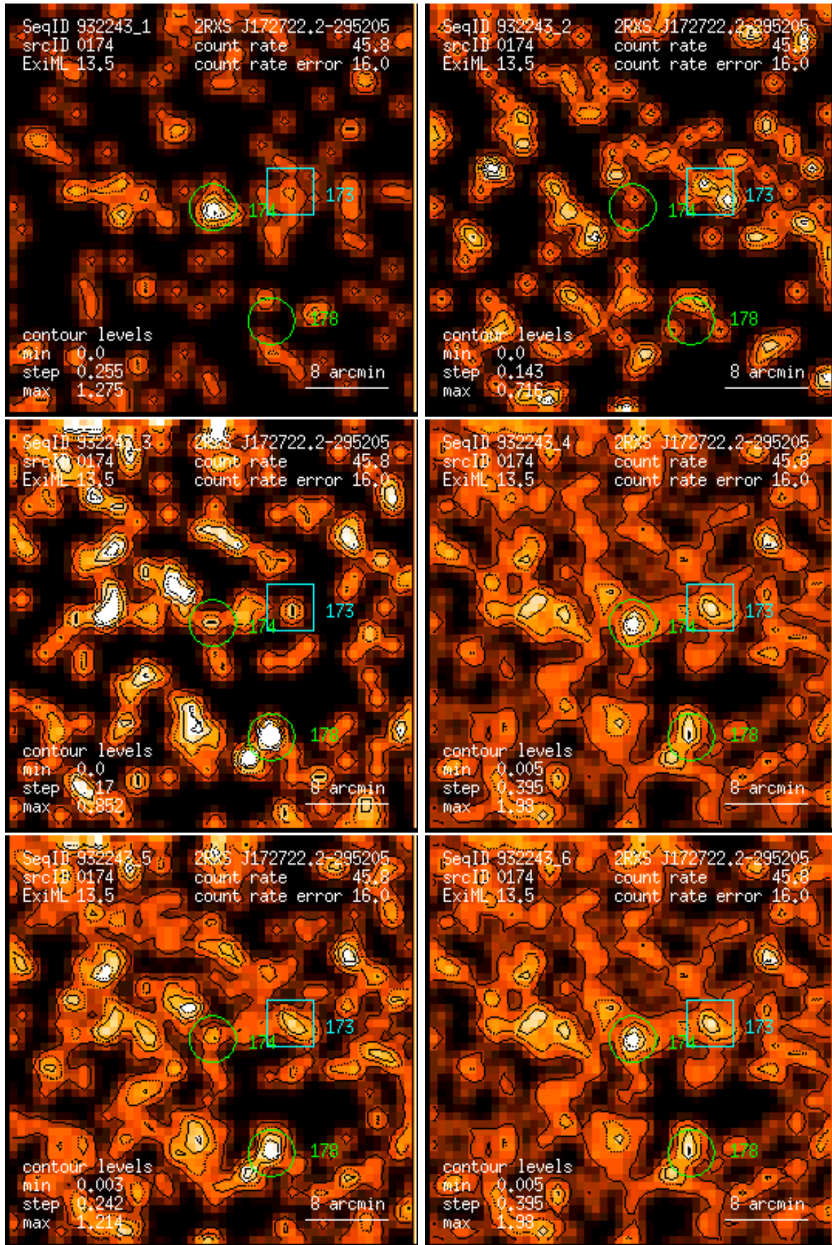
Figure 174: RASS 932243: detection 0174: band rate images, Gaussian filter: (1) PSPC channels 11 – 41, (2) 52 – 90, (3) 91 – 201, (4) 11 – 235, (5) 52 – 201, (6) 11 – 201. Broad band rates in counts/ks. Band rate contour levels in counts/ks/arcmin 2 .
