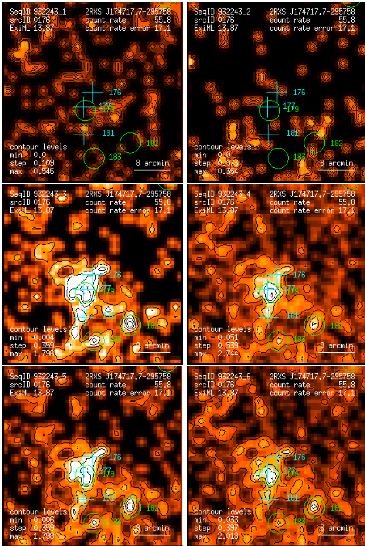
Figure 176: RASS 932243: detection 0176: band rate images, Gaussian filter: (1) PSPC channels 11 – 41, (2) 52 – 90, (3) 91 – 201, (4) 11 – 235, (5) 52 – 201, (6) 11 – 201. Broad band rates in counts/ks. Band rate contour levels in counts/ks/arcmin 2 .
