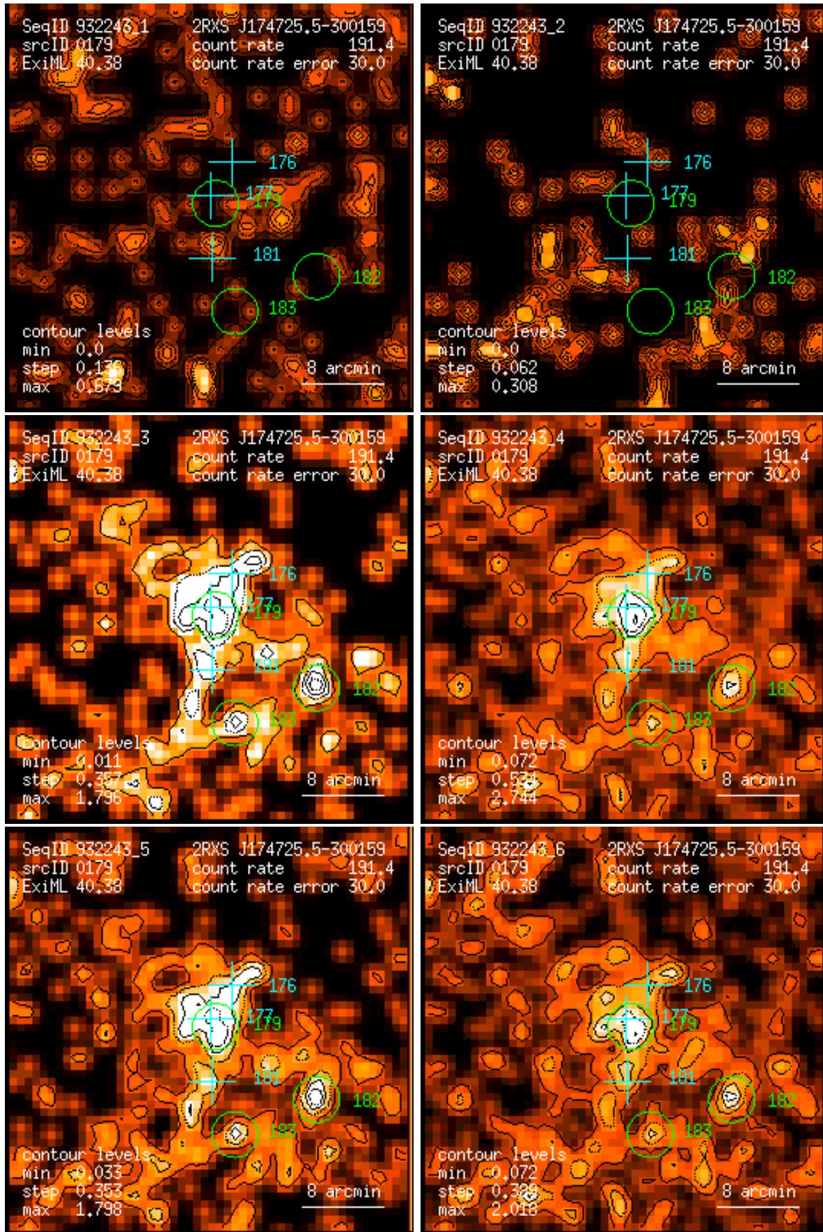
Figure 179: RASS 932243: detection 0179: band rate images, Gaussian filter: (1) PSPC channels 11 – 41, (2) 52 – 90, (3) 91 – 201, (4) 11 – 235, (5) 52 – 201, (6) 11 – 201. Broad band rates in counts/ks. Band rate contour levels in counts/ks/arcmin 2 .
