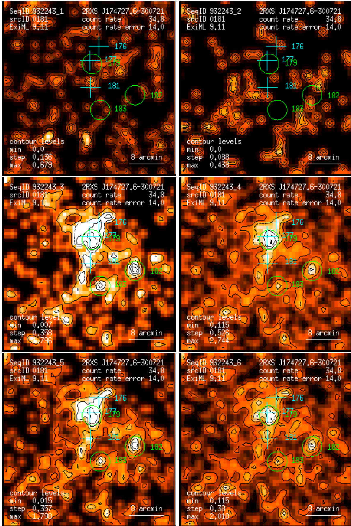
Figure 181: RASS 932243: detection 0181: band rate images, Gaussian filter: (1) PSPC channels 11 – 41, (2) 52 – 90, (3) 91 – 201, (4) 11 – 235, (5) 52 – 201, (6) 11 – 201. Broad band rates in counts/ks. Band rate contour levels in counts/ks/arcmin 2 .
