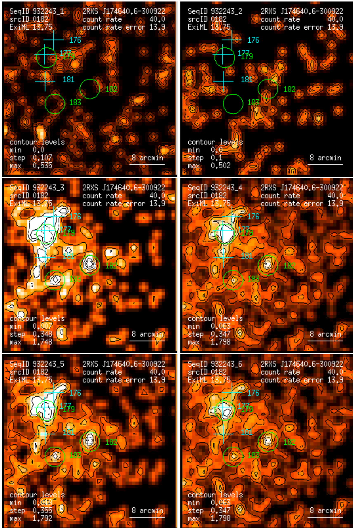
Figure 182: RASS 932243: detection 0182: band rate images, Gaussian filter: (1) PSPC channels 11 – 41, (2) 52 – 90, (3) 91 – 201, (4) 11 – 235, (5) 52 – 201, (6) 11 – 201. Broad band rates in counts/ks. Band rate contour levels in counts/ks/arcmin 2 .
