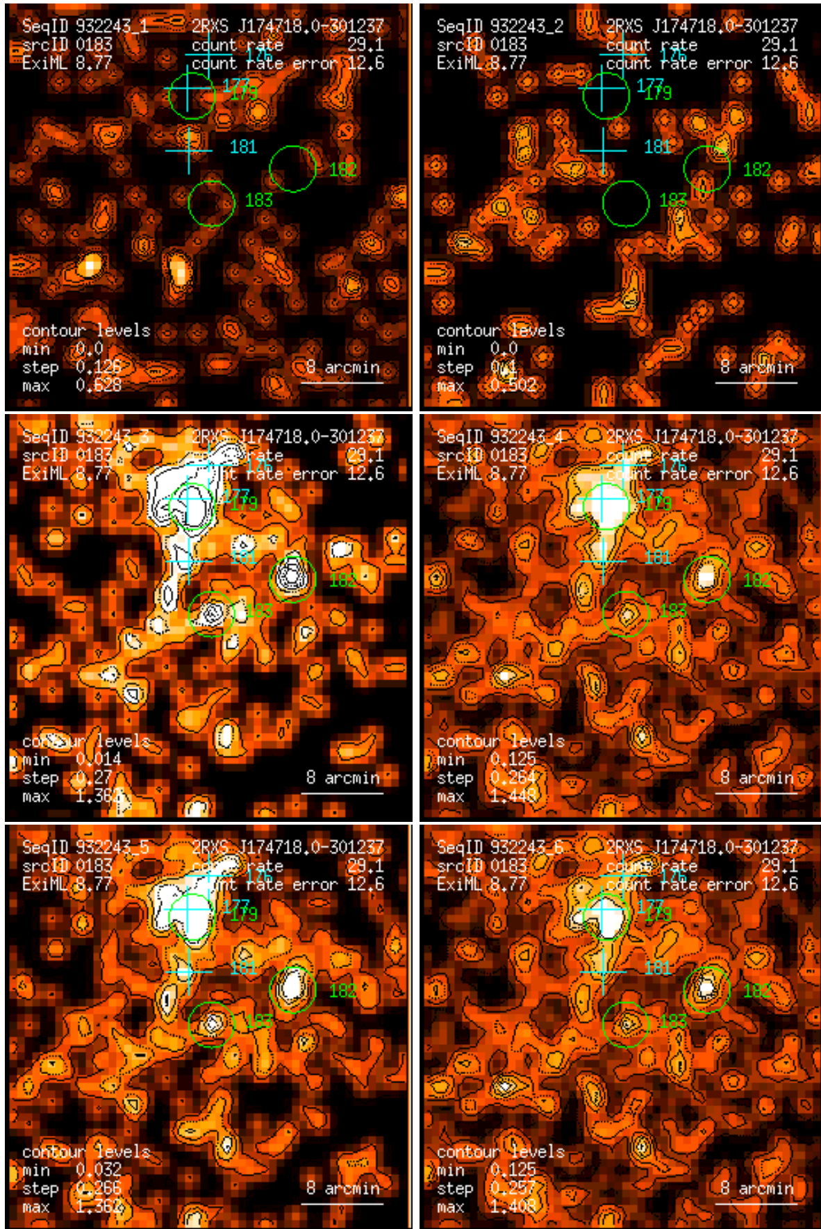
Figure 183: RASS 932243: detection 0183: band rate images, Gaussian filter: (1) PSPC channels 11 – 41, (2) 52 – 90, (3) 91 – 201, (4) 11 – 235, (5) 52 – 201, (6) 11 – 201. Broad band rates in counts/ks. Band rate contour levels in counts/ks/arcmin 2 .
