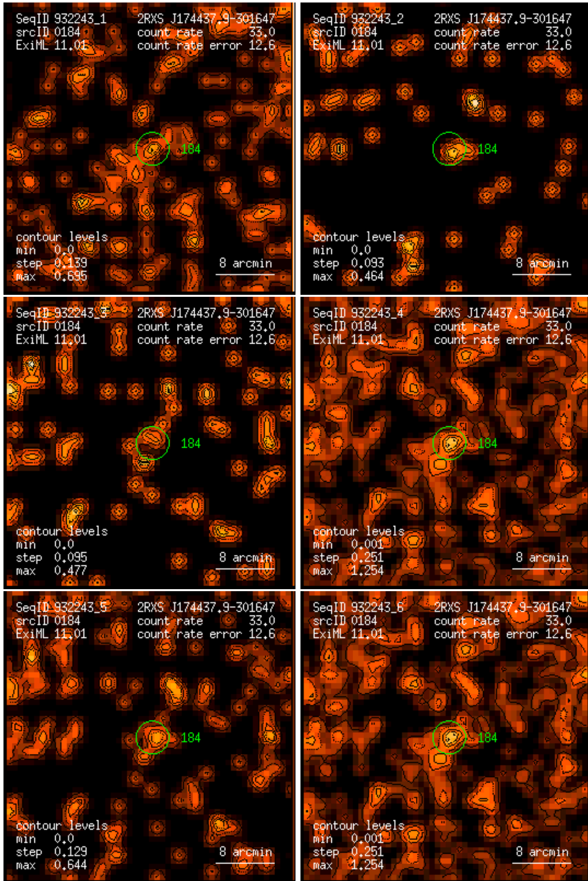
Figure 184: RASS 932243: detection 0184: band rate images, Gaussian filter: (1) PSPC channels 11 – 41, (2) 52 – 90, (3) 91 – 201, (4) 11 – 235, (5) 52 – 201, (6) 11 – 201. Broad band rates in counts/ks. Band rate contour levels in counts/ks/arcmin 2 .
