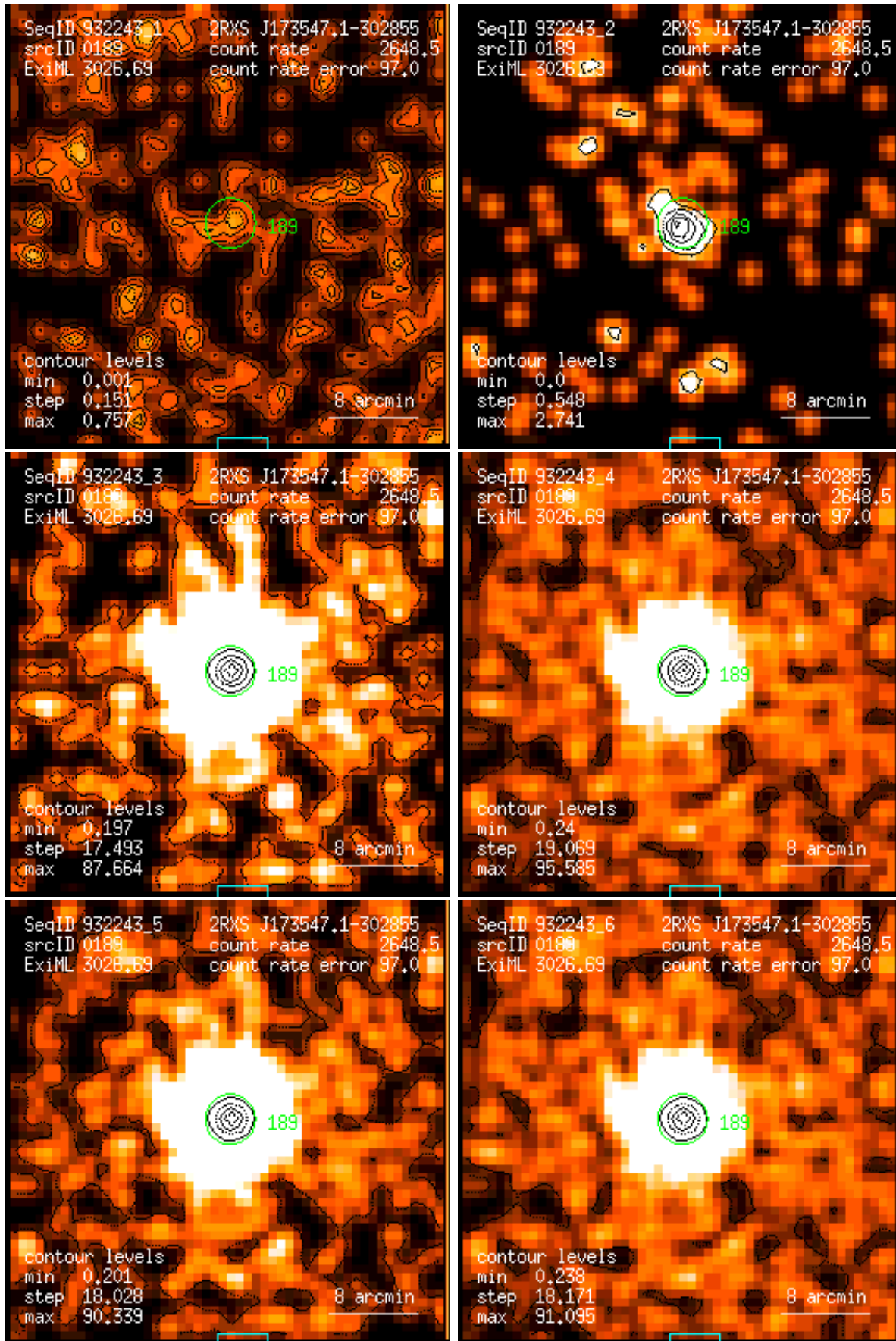
Figure 189: RASS 932243: detection 0189: band rate images, Gaussian filter: (1) PSPC channels 11 – 41, (2) 52 – 90, (3) 91 – 201, (4) 11 – 235, (5) 52 – 201, (6) 11 – 201. Broad band rates in counts/ks. Band rate contour levels in counts/ks/arcmin 2 .
