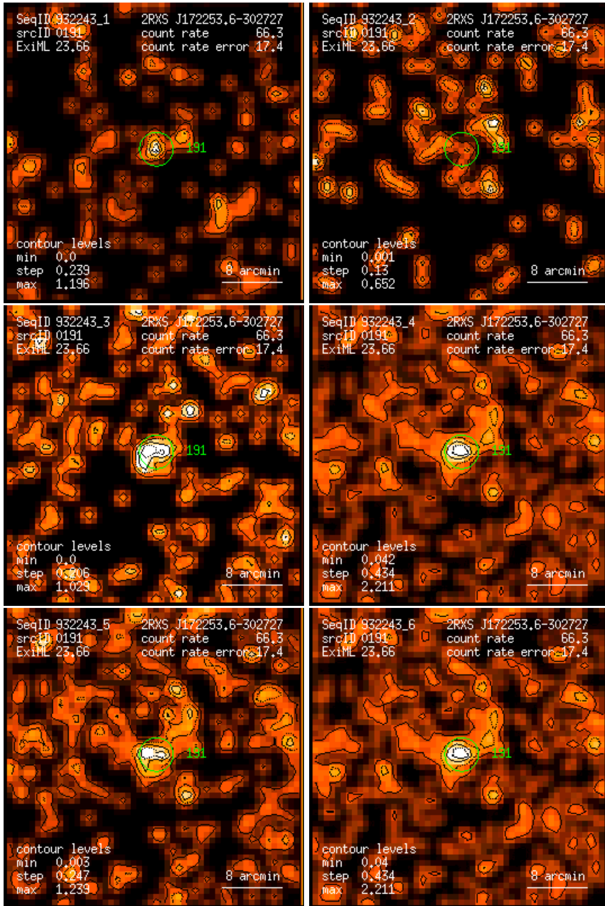
Figure 191: RASS 932243: detection 0191: band rate images, Gaussian filter: (1) PSPC channels 11 – 41, (2) 52 – 90, (3) 91 – 201, (4) 11 – 235, (5) 52 – 201, (6) 11 – 201. Broad band rates in counts/ks. Band rate contour levels in counts/ks/arcmin 2 .
