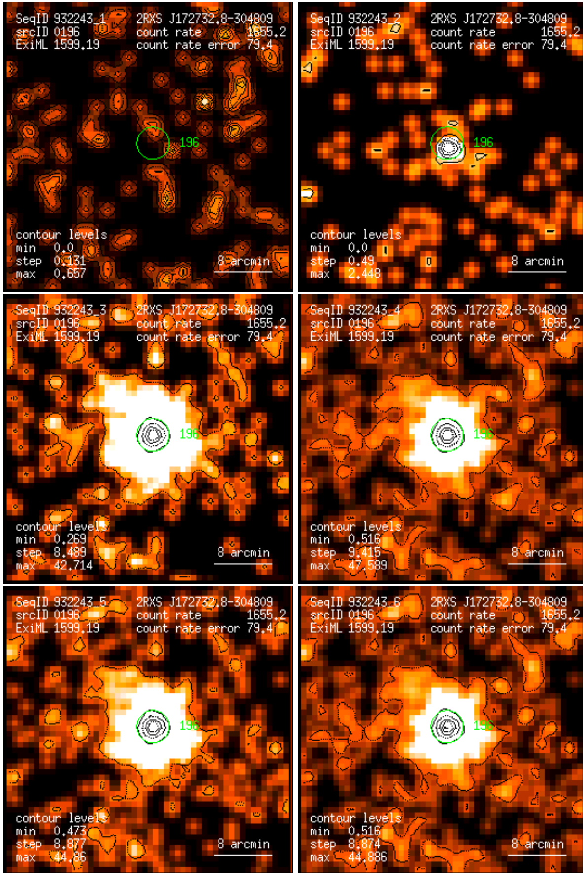
Figure 196: RASS 932243: detection 0196: band rate images, Gaussian filter: (1) PSPC channels 11 – 41, (2) 52 – 90, (3) 91 – 201, (4) 11 – 235, (5) 52 – 201, (6) 11 – 201. Broad band rates in counts/ks. Band rate contour levels in counts/ks/arcmin 2 .
