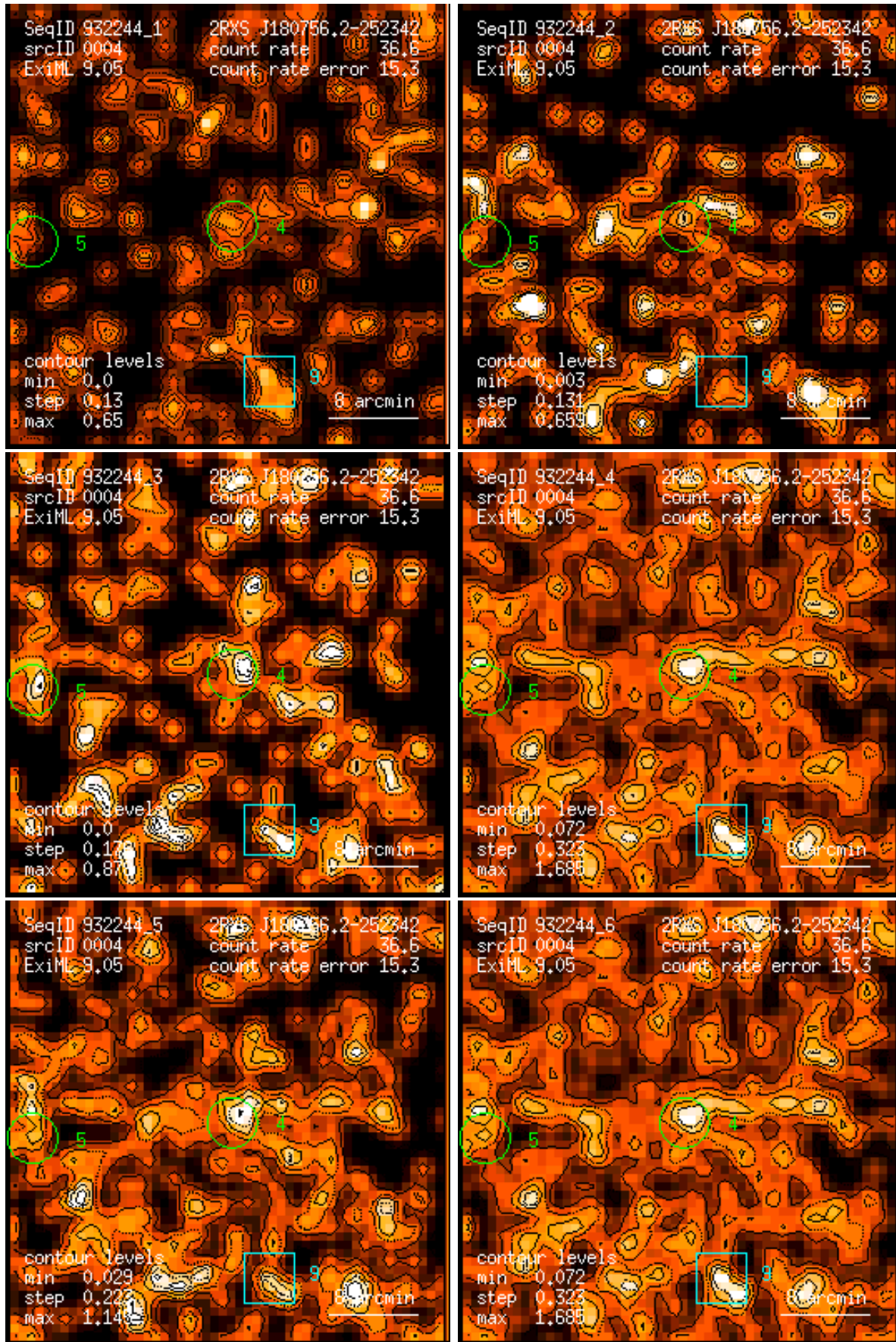
Figure 4: RASS 932244: detection 0004: band rate images, Gaussian filter: (1) PSPC channels 11 – 41, (2) 52 – 90, (3) 91 – 201, (4) 11 – 235, (5) 52 – 201, (6) 11 – 201. Broad band rates in counts/ks. Band rate contour levels in counts/ks/arcmin 2 .
