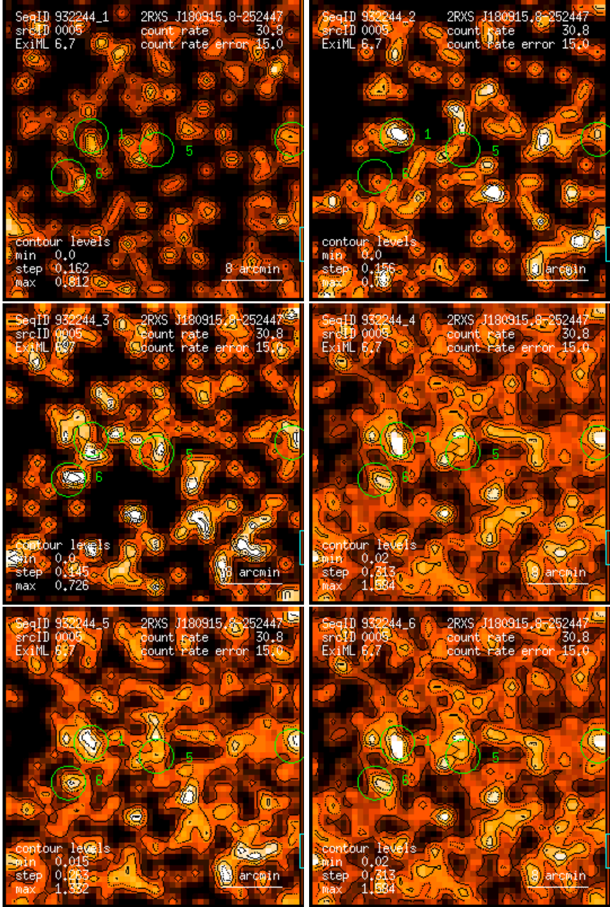
Figure 5: RASS 932244: detection 0005: band rate images, Gaussian filter: (1) PSPC channels 11 – 41, (2) 52 – 90, (3) 91 – 201, (4) 11 – 235, (5) 52 – 201, (6) 11 – 201. Broad band rates in counts/ks. Band rate contour levels in counts/ks/arcmin 2 .
