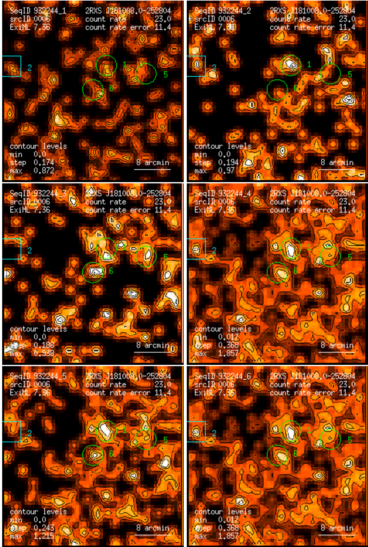
Figure 6: RASS 932244: detection 0006: band rate images, Gaussian filter: (1) PSPC channels 11 – 41, (2) 52 – 90, (3) 91 – 201, (4) 11 – 235, (5) 52 – 201, (6) 11 – 201. Broad band rates in counts/ks. Band rate contour levels in counts/ks/arcmin 2 .
