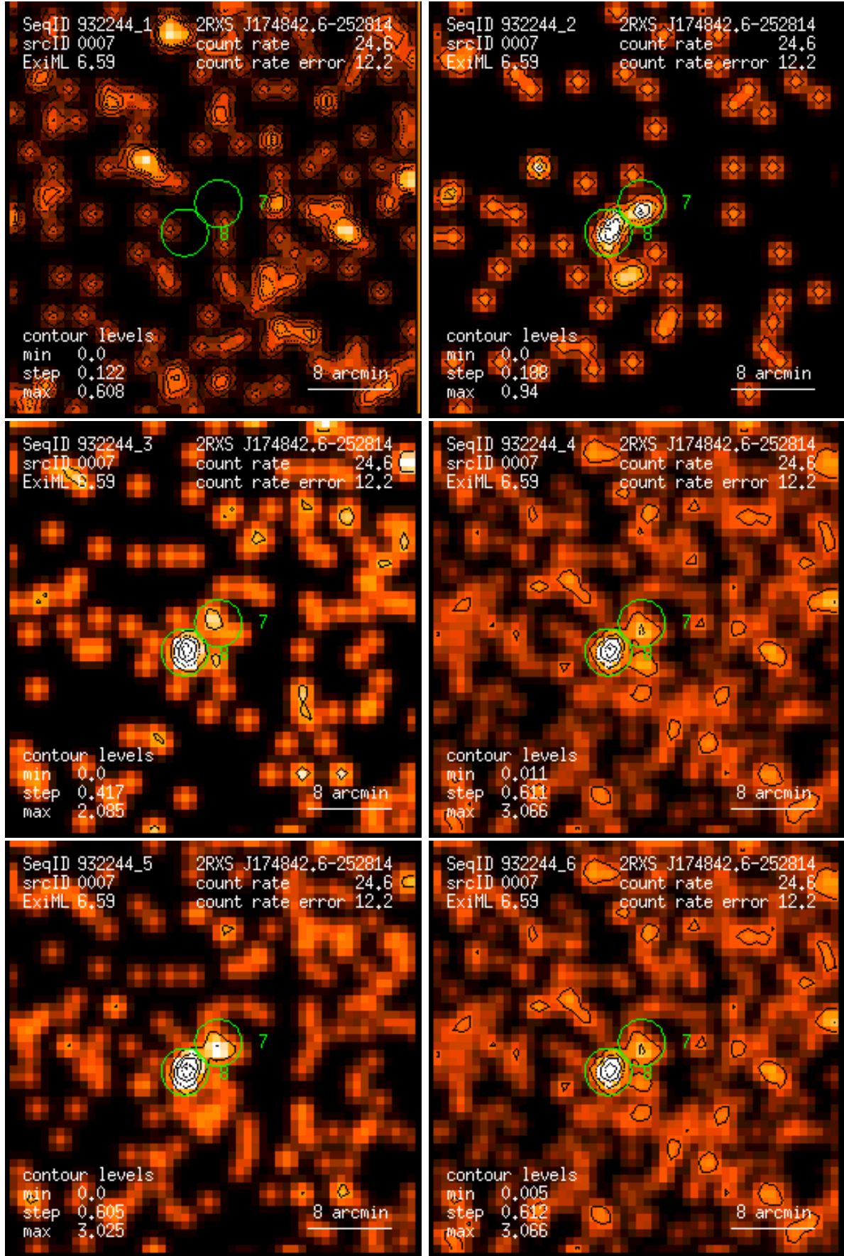
Figure 7: RASS 932244: detection 0007: band rate images, Gaussian filter: (1) PSPC channels 11 – 41, (2) 52 – 90, (3) 91 – 201, (4) 11 – 235, (5) 52 – 201, (6) 11 – 201. Broad band rates in counts/ks. Band rate contour levels in counts/ks/arcmin 2 .
