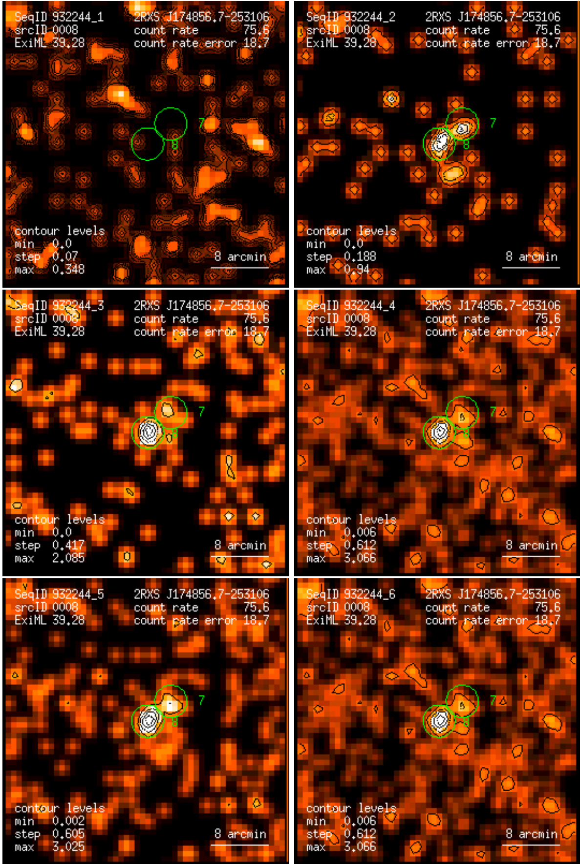
Figure 8: RASS 932244: detection 0008: band rate images, Gaussian filter: (1) PSPC channels 11 – 41, (2) 52 – 90, (3) 91 – 201, (4) 11 – 235, (5) 52 – 201, (6) 11 – 201. Broad band rates in counts/ks. Band rate contour levels in counts/ks/arcmin 2 .
