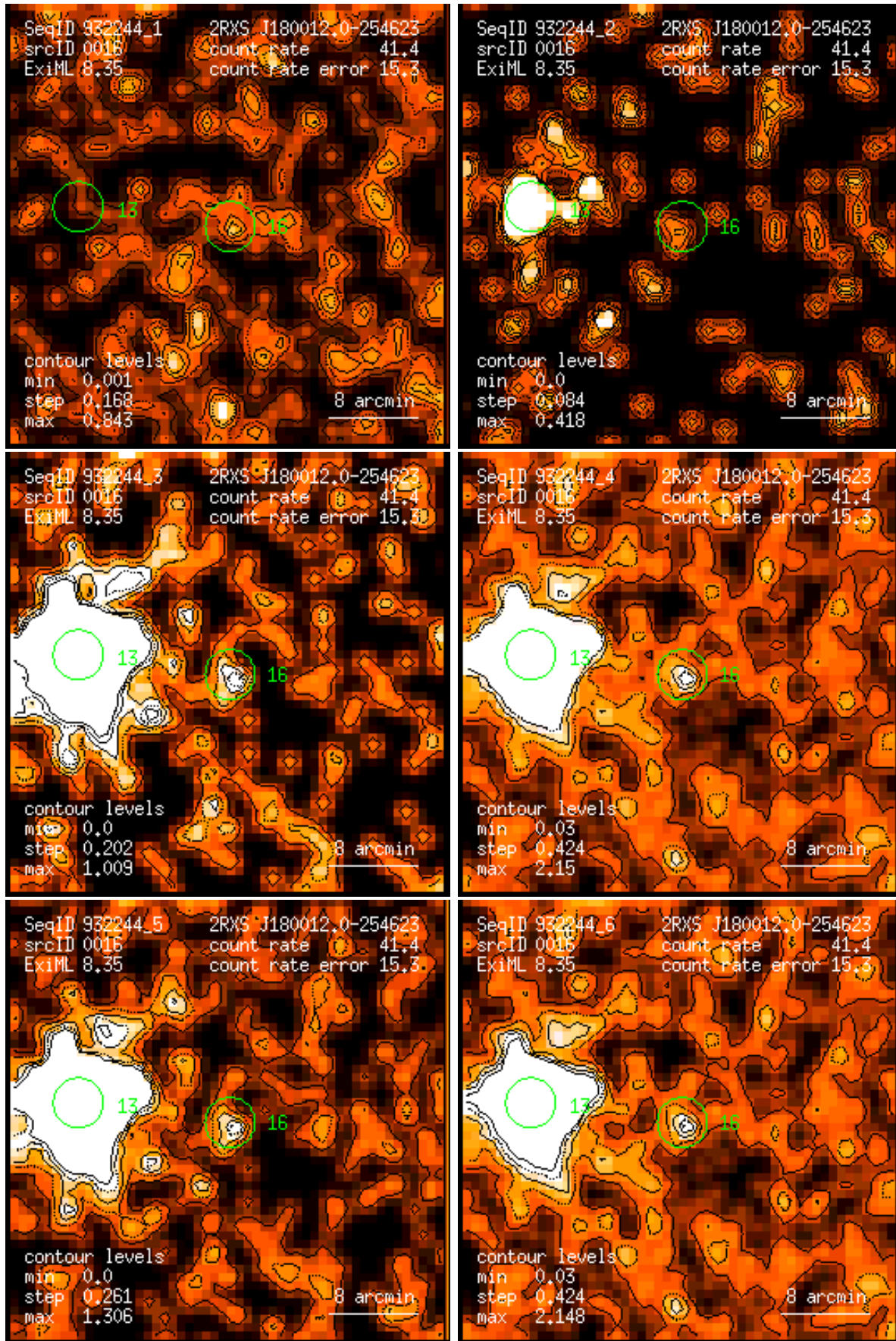
Figure 16: RASS 932244: detection 0016: band rate images, Gaussian filter: (1) PSPC channels 11 – 41, (2) 52 – 90, (3) 91 – 201, (4) 11 – 235, (5) 52 – 201, (6) 11 – 201. Broad band rates in counts/ks. Band rate contour levels in counts/ks/arcmin 2 .
