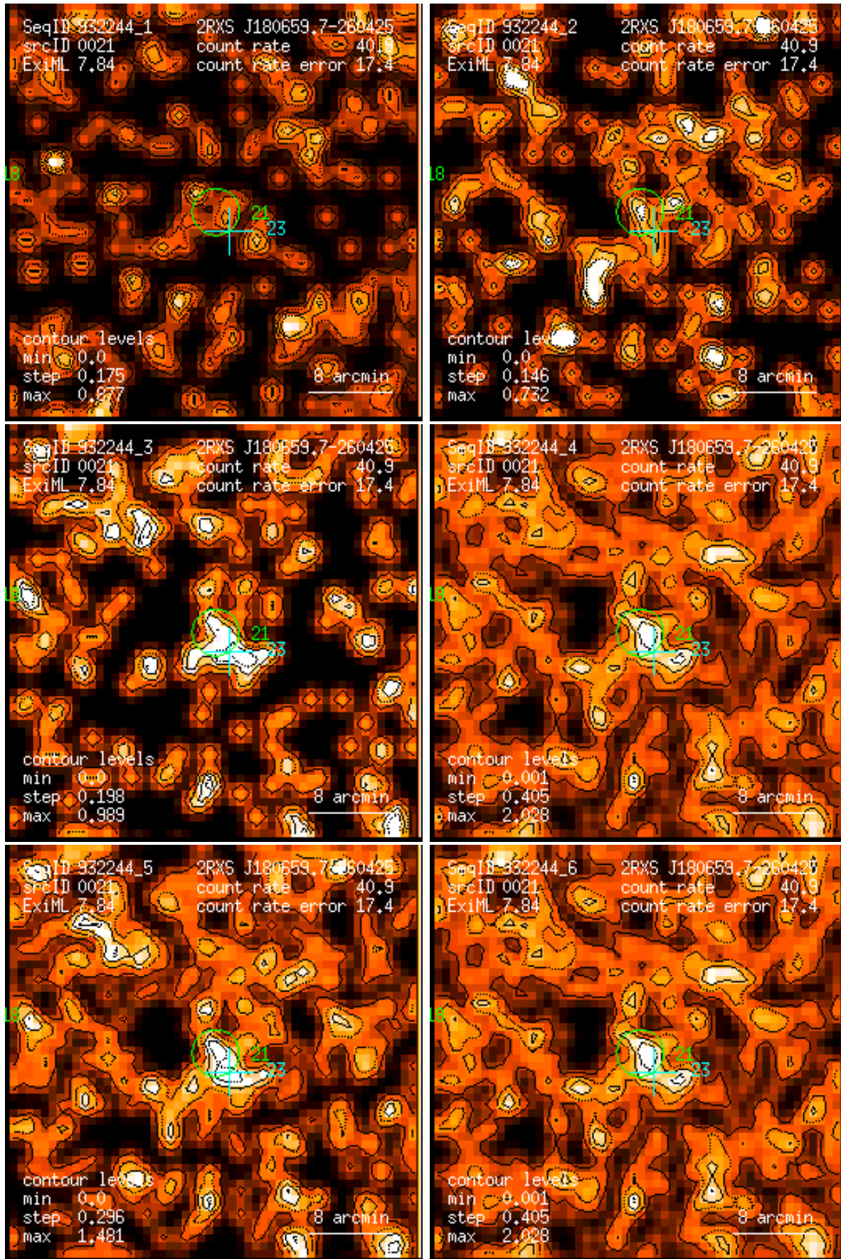
Figure 21: RASS 932244: detection 0021: band rate images, Gaussian filter: (1) PSPC channels 11 – 41, (2) 52 – 90, (3) 91 – 201, (4) 11 – 235, (5) 52 – 201, (6) 11 – 201. Broad band rates in counts/ks. Band rate contour levels in counts/ks/arcmin 2 .
