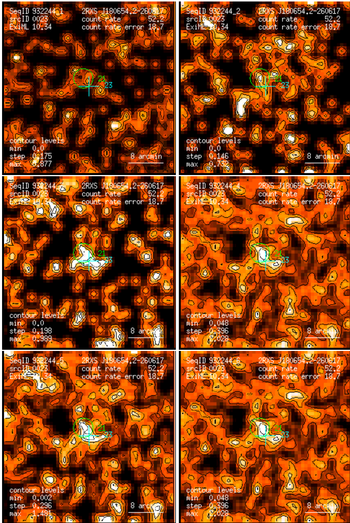
Figure 23: RASS 932244: detection 0023: band rate images, Gaussian filter: (1) PSPC channels 11 – 41, (2) 52 – 90, (3) 91 – 201, (4) 11 – 235, (5) 52 – 201, (6) 11 – 201. Broad band rates in counts/ks. Band rate contour levels in counts/ks/arcmin 2 .
