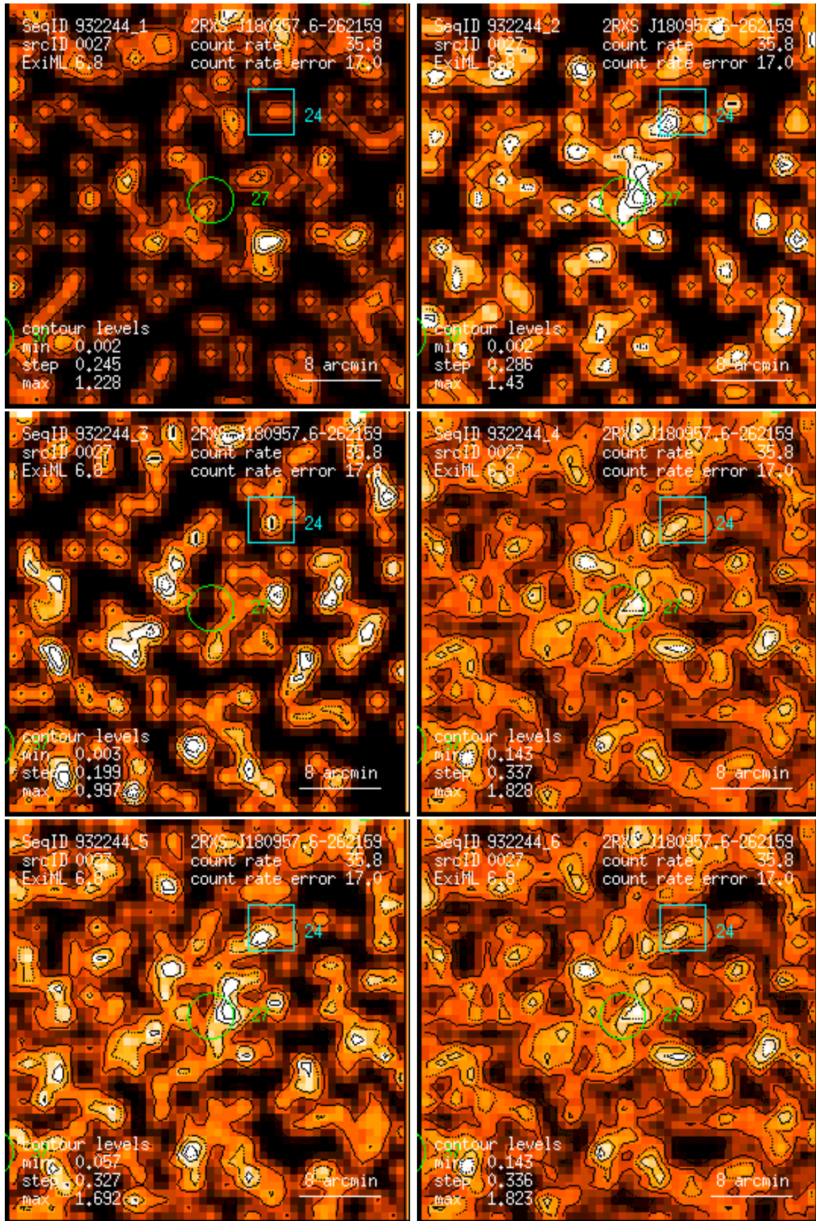
Figure 27: RASS 932244: detection 0027: band rate images, Gaussian filter: (1) PSPC channels 11 – 41, (2) 52 – 90, (3) 91 – 201, (4) 11 – 235, (5) 52 – 201, (6) 11 – 201. Broad band rates in counts/ks. Band rate contour levels in counts/ks/arcmin 2 .
