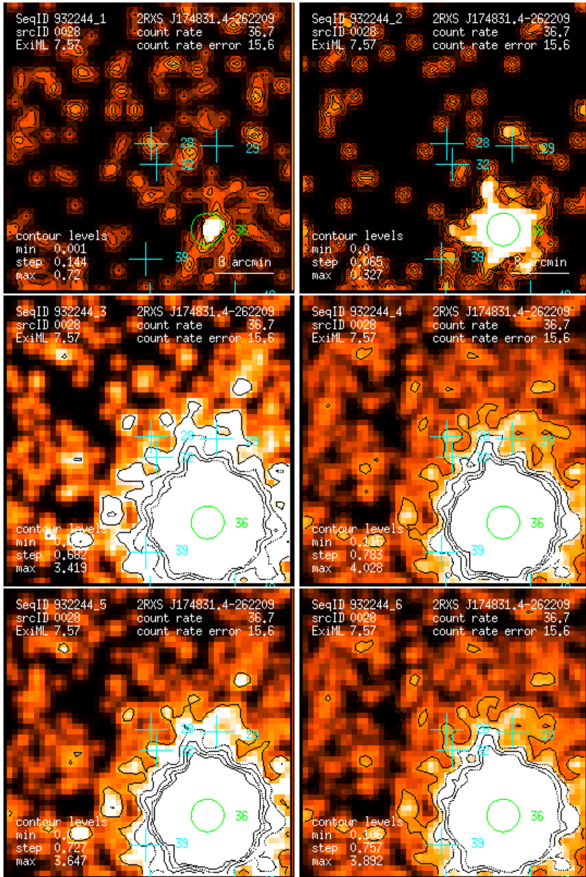
Figure 28: RASS 932244: detection 0028: band rate images, Gaussian filter: (1) PSPC channels 11 – 41, (2) 52 – 90, (3) 91 – 201, (4) 11 – 235, (5) 52 – 201, (6) 11 – 201. Broad band rates in counts/ks. Band rate contour levels in counts/ks/arcmin 2 .
