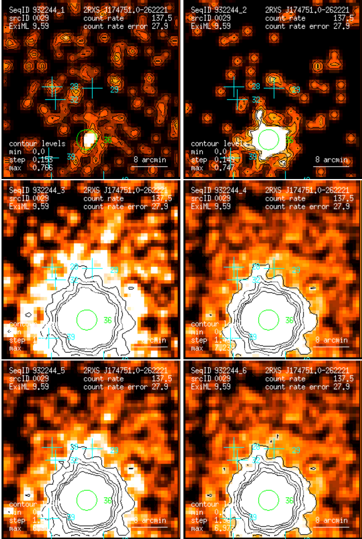
Figure 29: RASS 932244: detection 0029: band rate images, Gaussian filter: (1) PSPC channels 11 – 41, (2) 52 – 90, (3) 91 – 201, (4) 11 – 235, (5) 52 – 201, (6) 11 – 201. Broad band rates in counts/ks. Band rate contour levels in counts/ks/arcmin 2 .
