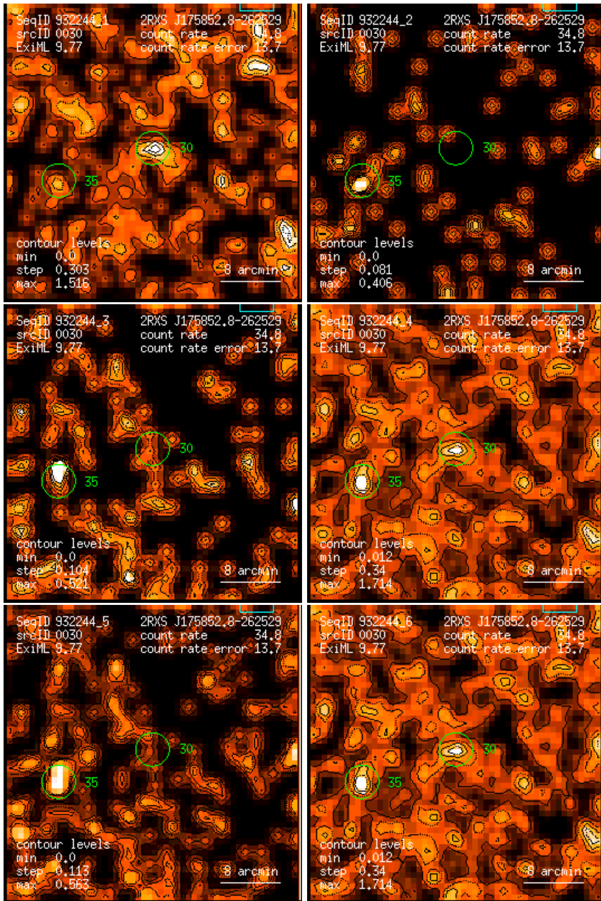
Figure 30: RASS 932244: detection 0030: band rate images, Gaussian filter: (1) PSPC channels 11 – 41, (2) 52 – 90, (3) 91 – 201, (4) 11 – 235, (5) 52 – 201, (6) 11 – 201. Broad band rates in counts/ks. Band rate contour levels in counts/ks/arcmin 2 .
