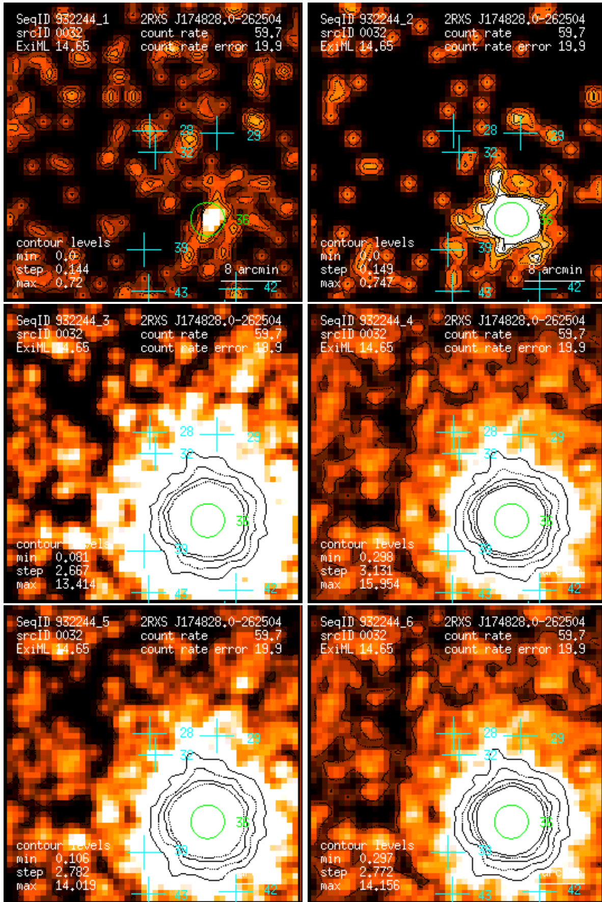
Figure 32: RASS 932244: detection 0032: band rate images, Gaussian filter: (1) PSPC channels 11 – 41, (2) 52 – 90, (3) 91 – 201, (4) 11 – 235, (5) 52 – 201, (6) 11 – 201. Broad band rates in counts/ks. Band rate contour levels in counts/ks/arcmin 2 .
