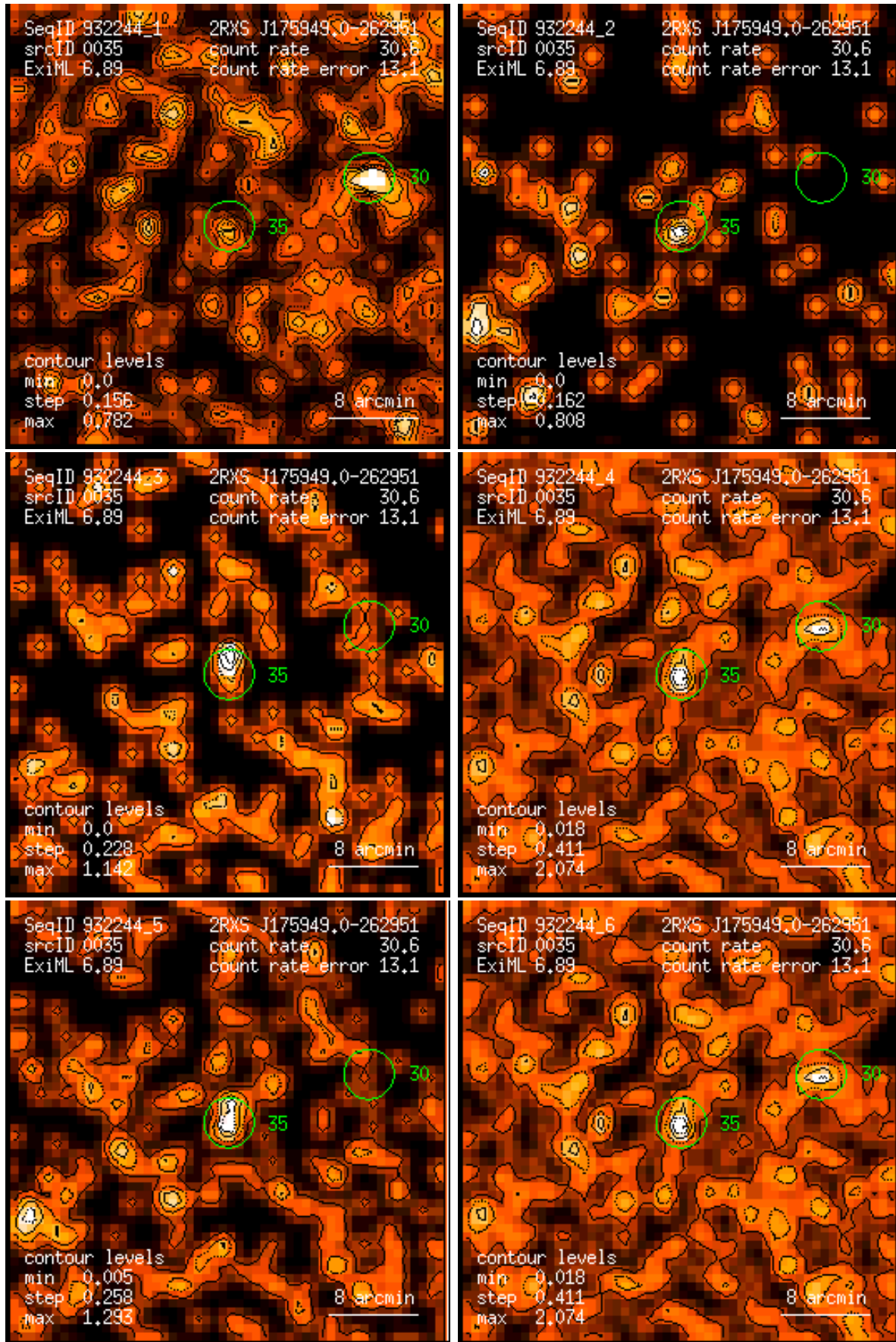
Figure 35: RASS 932244: detection 0035: band rate images, Gaussian filter: (1) PSPC channels 11 – 41, (2) 52 – 90, (3) 91 – 201, (4) 11 – 235, (5) 52 – 201, (6) 11 – 201. Broad band rates in counts/ks. Band rate contour levels in counts/ks/arcmin 2 .
