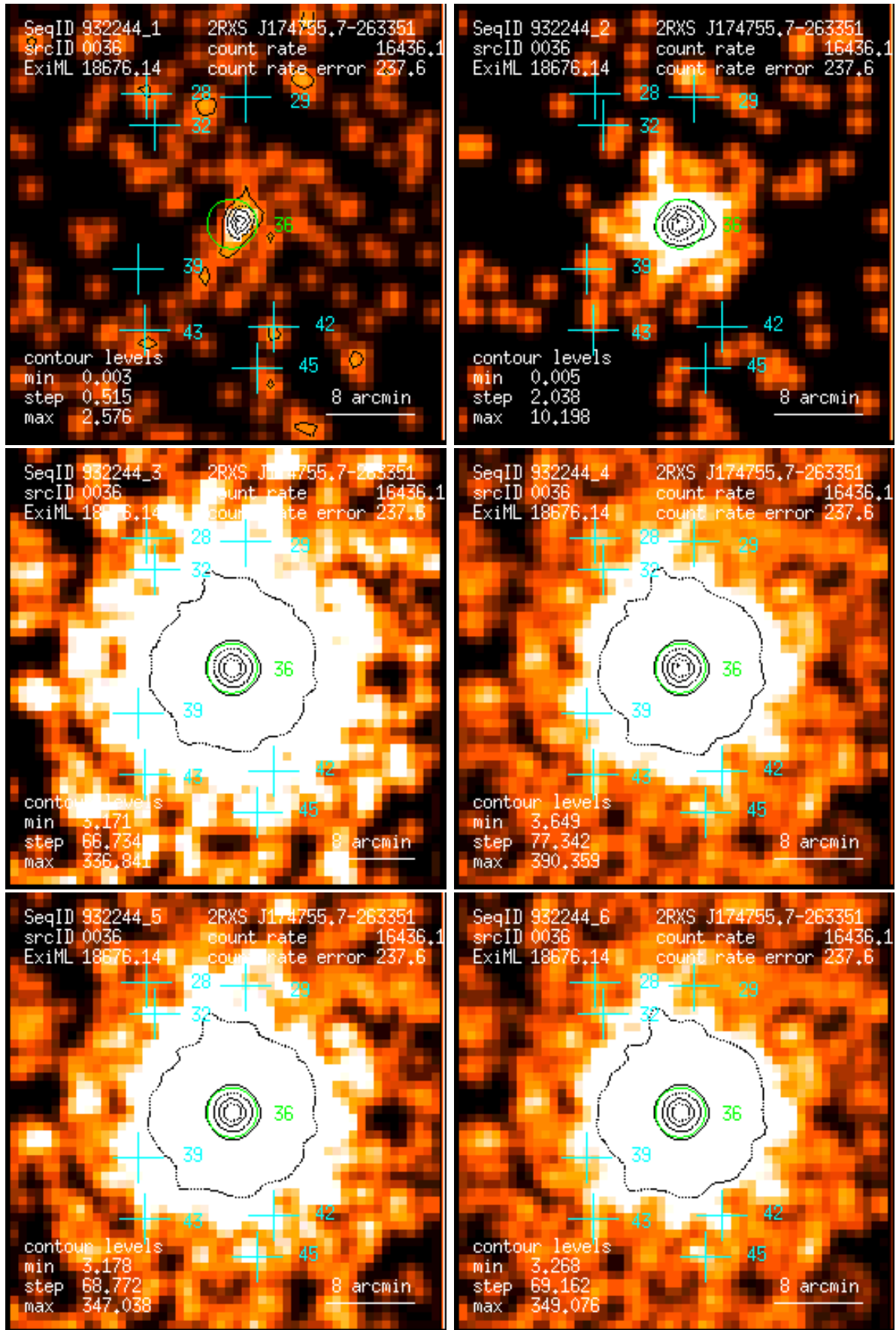
Figure 36: RASS 932244: detection 0036: band rate images, Gaussian filter: (1) PSPC channels 11 – 41, (2) 52 – 90, (3) 91 – 201, (4) 11 – 235, (5) 52 – 201, (6) 11 – 201. Broad band rates in counts/ks. Band rate contour levels in counts/ks/arcmin 2 .
