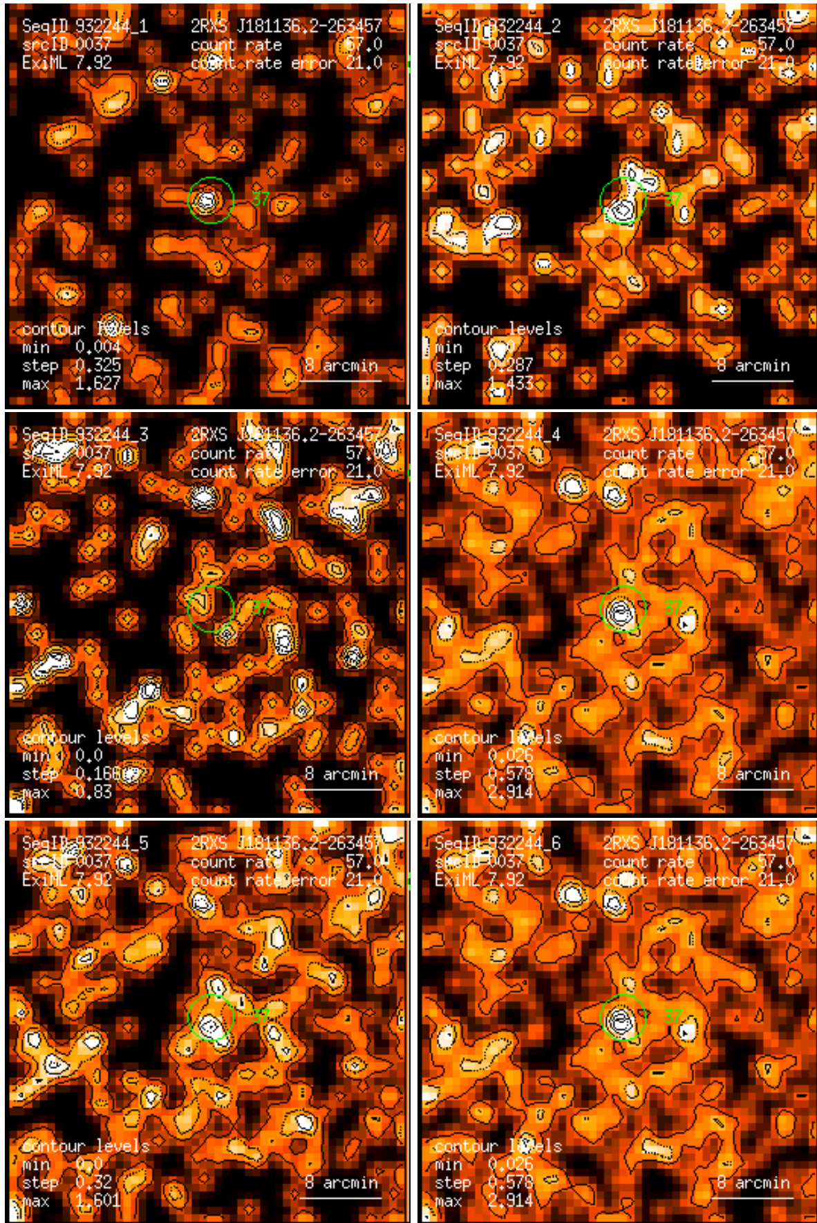
Figure 37: RASS 932244: detection 0037: band rate images, Gaussian filter: (1) PSPC channels 11 – 41, (2) 52 – 90, (3) 91 – 201, (4) 11 – 235, (5) 52 – 201, (6) 11 – 201. Broad band rates in counts/ks. Band rate contour levels in counts/ks/arcmin 2 .
