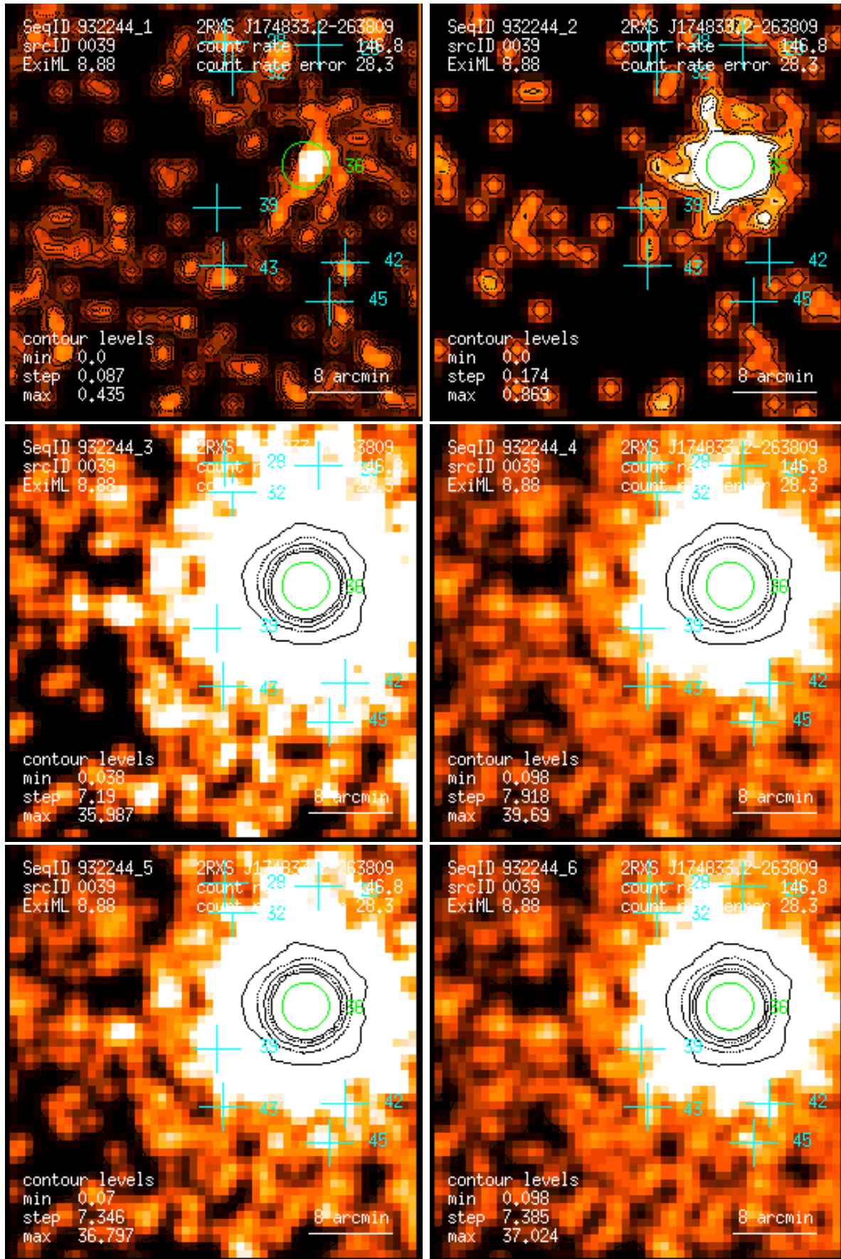
Figure 39: RASS 932244: detection 0039: band rate images, Gaussian filter: (1) PSPC channels 11 – 41, (2) 52 – 90, (3) 91 – 201, (4) 11 – 235, (5) 52 – 201, (6) 11 – 201. Broad band rates in counts/ks. Band rate contour levels in counts/ks/arcmin 2 .
