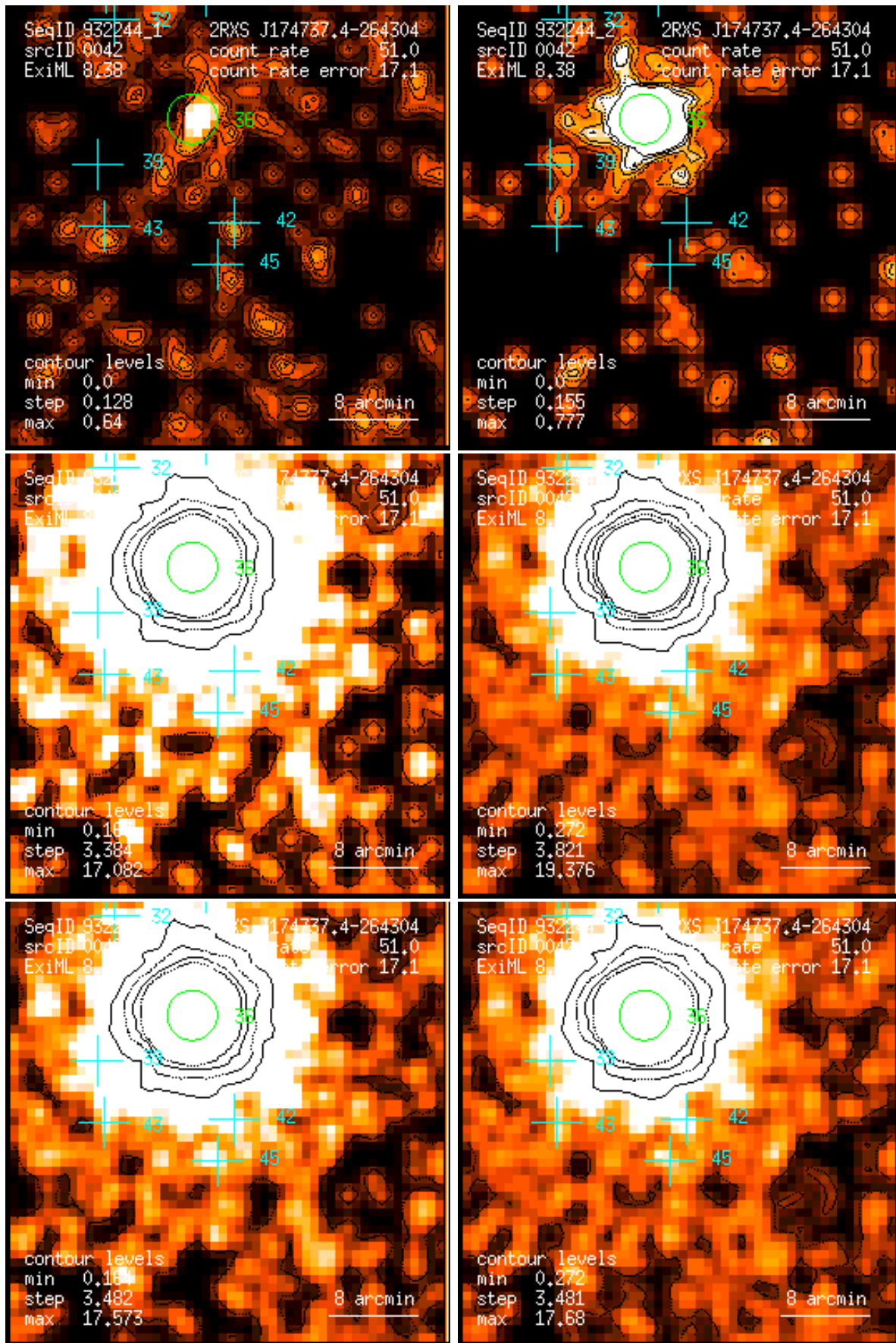
Figure 42: RASS 932244: detection 0042: band rate images, Gaussian filter: (1) PSPC channels 11 – 41, (2) 52 – 90, (3) 91 – 201, (4) 11 – 235, (5) 52 – 201, (6) 11 – 201. Broad band rates in counts/ks. Band rate contour levels in counts/ks/arcmin 2 .
