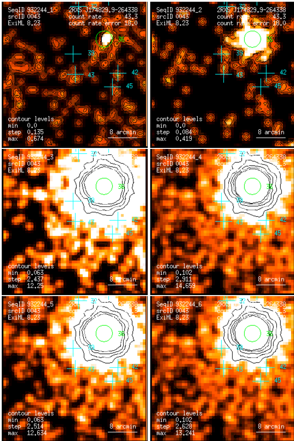
Figure 43: RASS 932244: detection 0043: band rate images, Gaussian filter: (1) PSPC channels 11 – 41, (2) 52 – 90, (3) 91 – 201, (4) 11 – 235, (5) 52 – 201, (6) 11 – 201. Broad band rates in counts/ks. Band rate contour levels in counts/ks/arcmin 2 .
