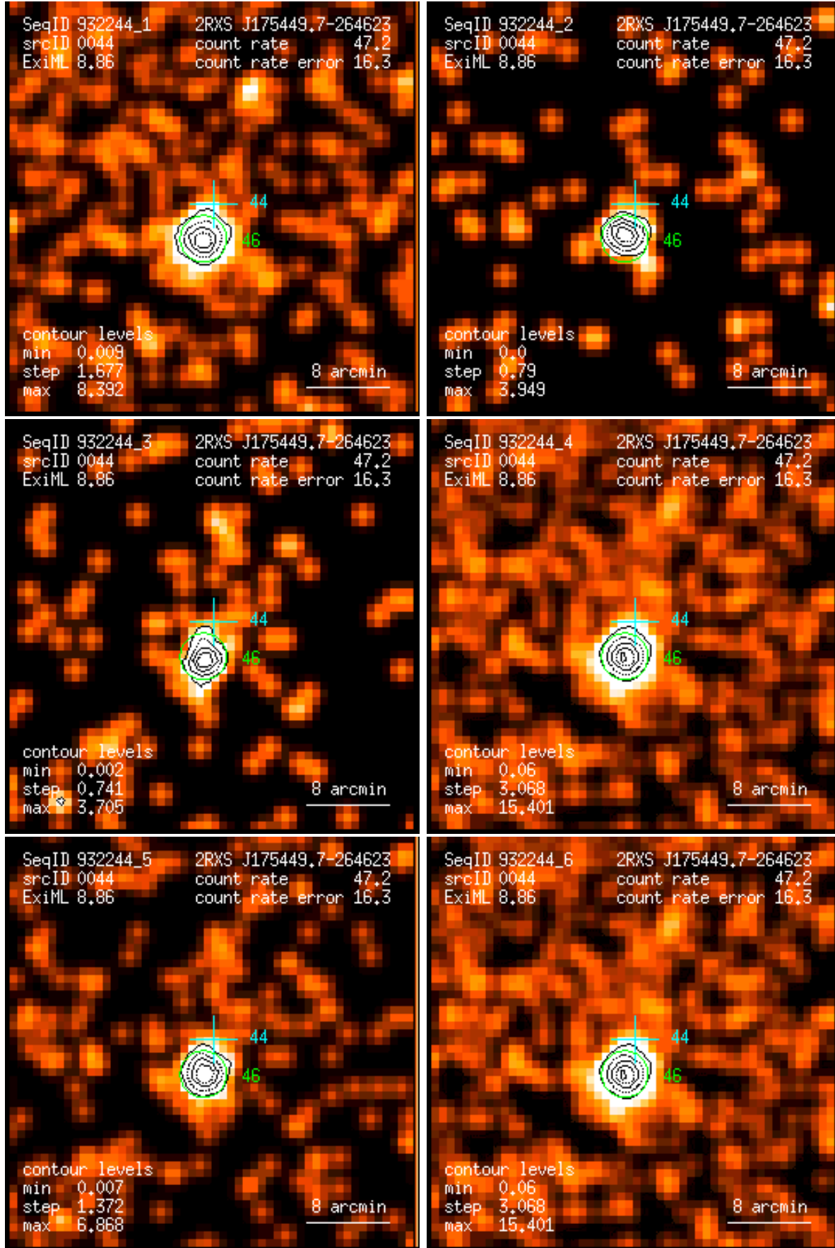
Figure 44: RASS 932244: detection 0044: band rate images, Gaussian filter: (1) PSPC channels 11 – 41, (2) 52 – 90, (3) 91 – 201, (4) 11 – 235, (5) 52 – 201, (6) 11 – 201. Broad band rates in counts/ks. Band rate contour levels in counts/ks/arcmin 2 .
