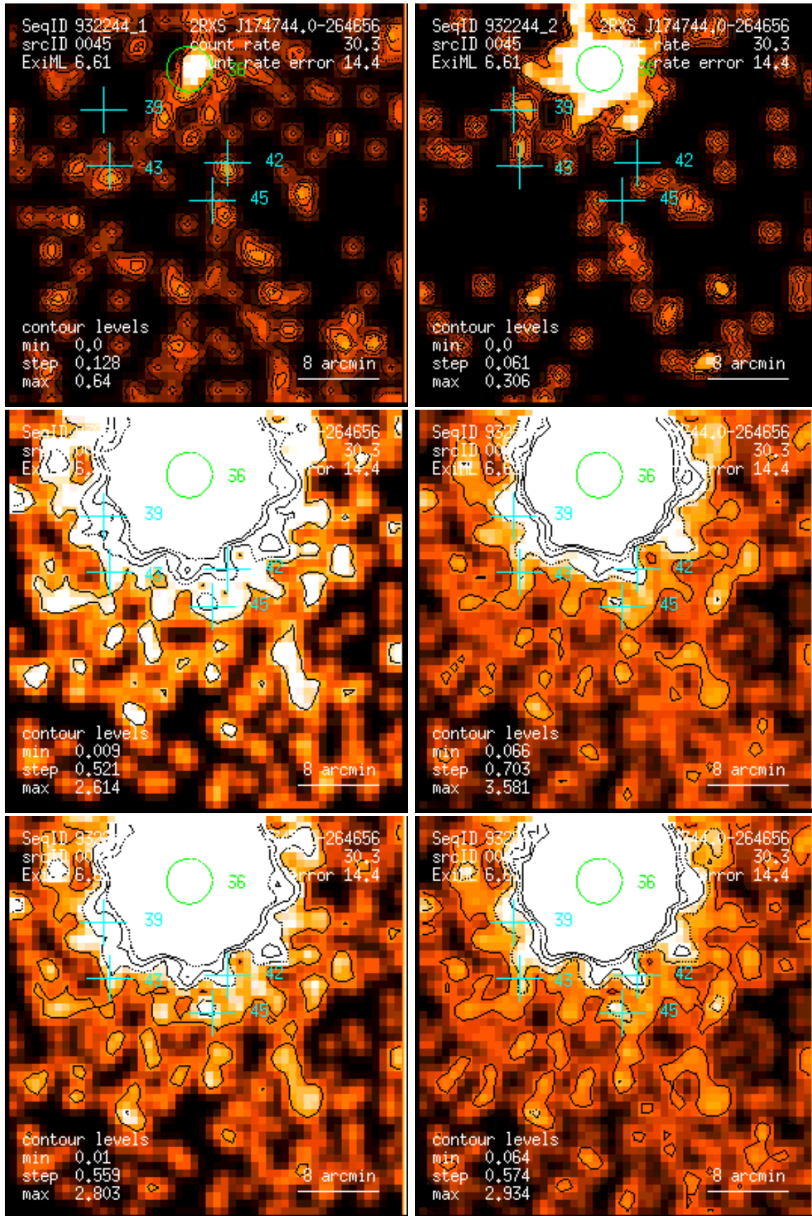
Figure 45: RASS 932244: detection 0045: band rate images, Gaussian filter: (1) PSPC channels 11 – 41, (2) 52 – 90, (3) 91 – 201, (4) 11 – 235, (5) 52 – 201, (6) 11 – 201. Broad band rates in counts/ks. Band rate contour levels in counts/ks/arcmin 2 .
