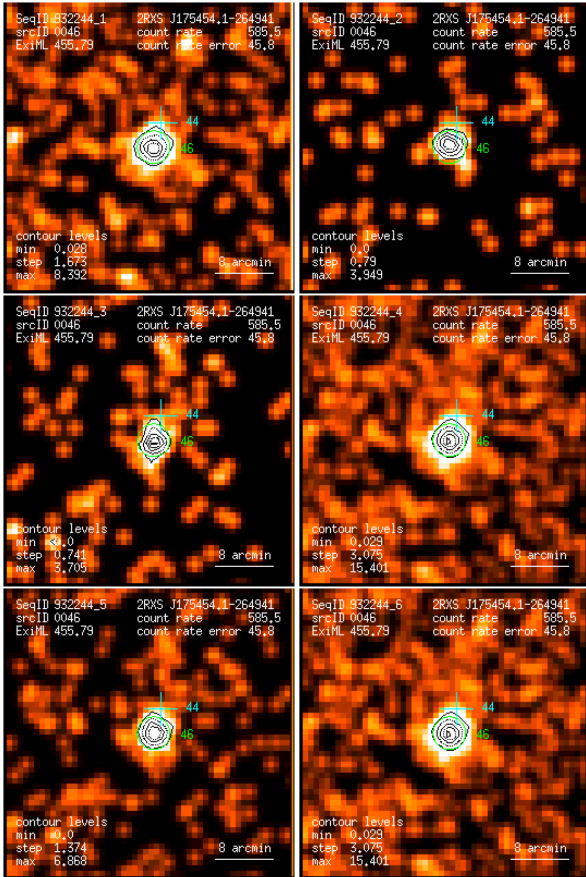
Figure 46: RASS 932244: detection 0046: band rate images, Gaussian filter: (1) PSPC channels 11 – 41, (2) 52 – 90, (3) 91 – 201, (4) 11 – 235, (5) 52 – 201, (6) 11 – 201. Broad band rates in counts/ks. Band rate contour levels in counts/ks/arcmin 2 .
