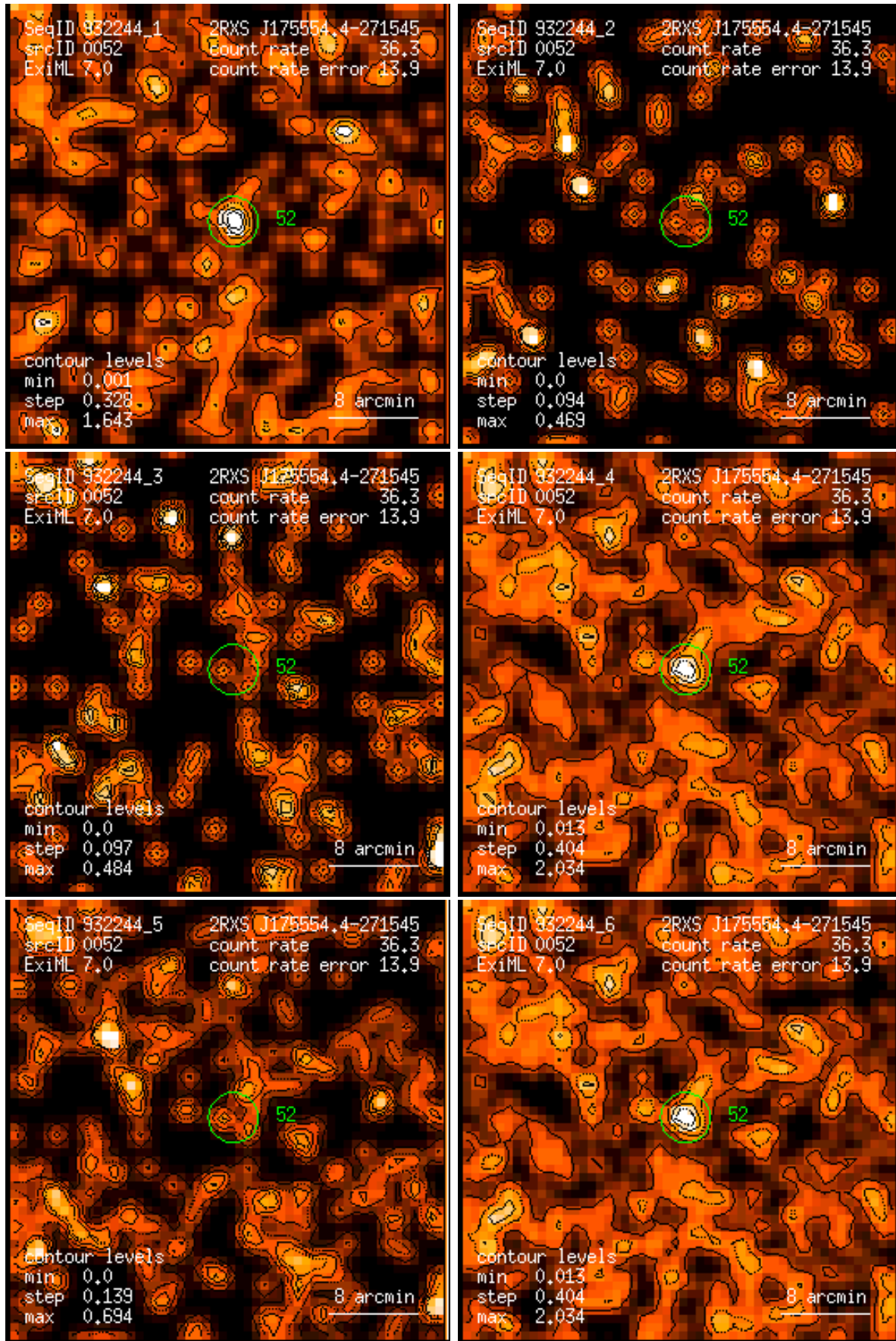
Figure 52: RASS 932244: detection 0052: band rate images, Gaussian filter: (1) PSPC channels 11 – 41, (2) 52 – 90, (3) 91 – 201, (4) 11 – 235, (5) 52 – 201, (6) 11 – 201. Broad band rates in counts/ks. Band rate contour levels in counts/ks/arcmin 2 .
