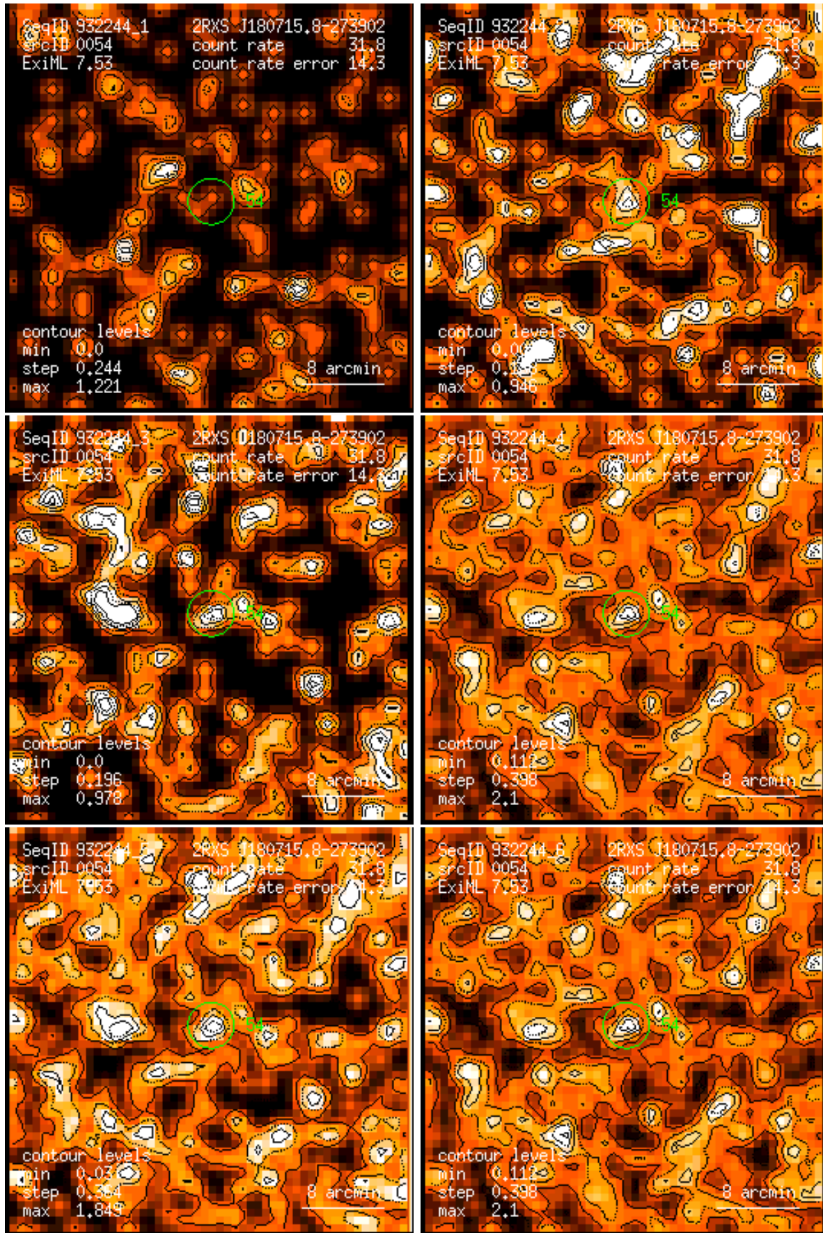
Figure 54: RASS 932244: detection 0054: band rate images, Gaussian filter: (1) PSPC channels 11 – 41, (2) 52 – 90, (3) 91 – 201, (4) 11 – 235, (5) 52 – 201, (6) 11 – 201. Broad band rates in counts/ks. Band rate contour levels in counts/ks/arcmin 2 .
