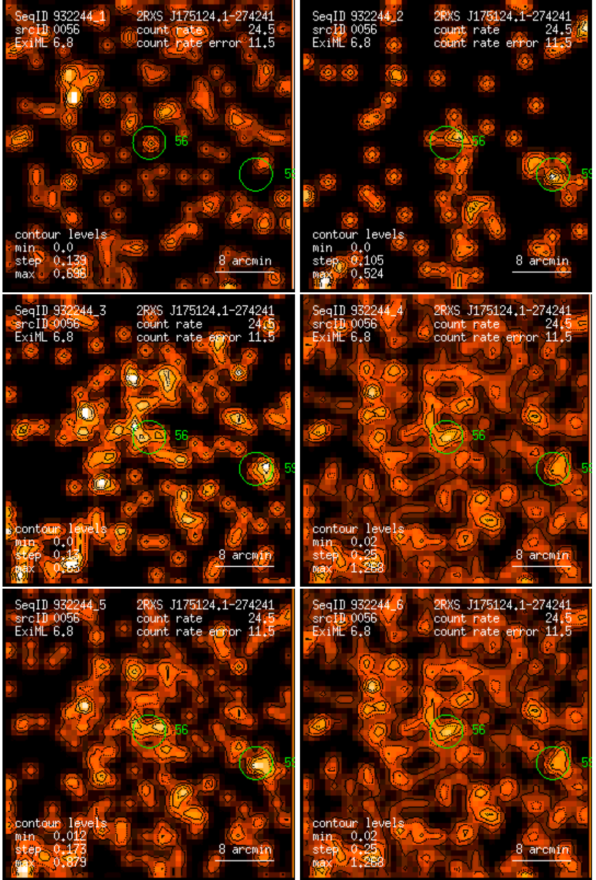
Figure 56: RASS 932244: detection 0056: band rate images, Gaussian filter: (1) PSPC channels 11 – 41, (2) 52 – 90, (3) 91 – 201, (4) 11 – 235, (5) 52 – 201, (6) 11 – 201. Broad band rates in counts/ks. Band rate contour levels in counts/ks/arcmin 2 .
