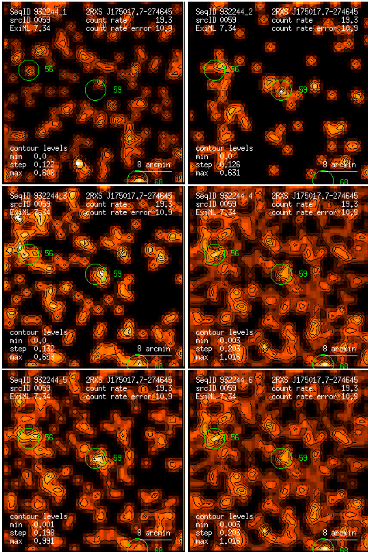
Figure 59: RASS 932244: detection 0059: band rate images, Gaussian filter: (1) PSPC channels 11 – 41, (2) 52 – 90, (3) 91 – 201, (4) 11 – 235, (5) 52 – 201, (6) 11 – 201. Broad band rates in counts/ks. Band rate contour levels in counts/ks/arcmin 2 .
