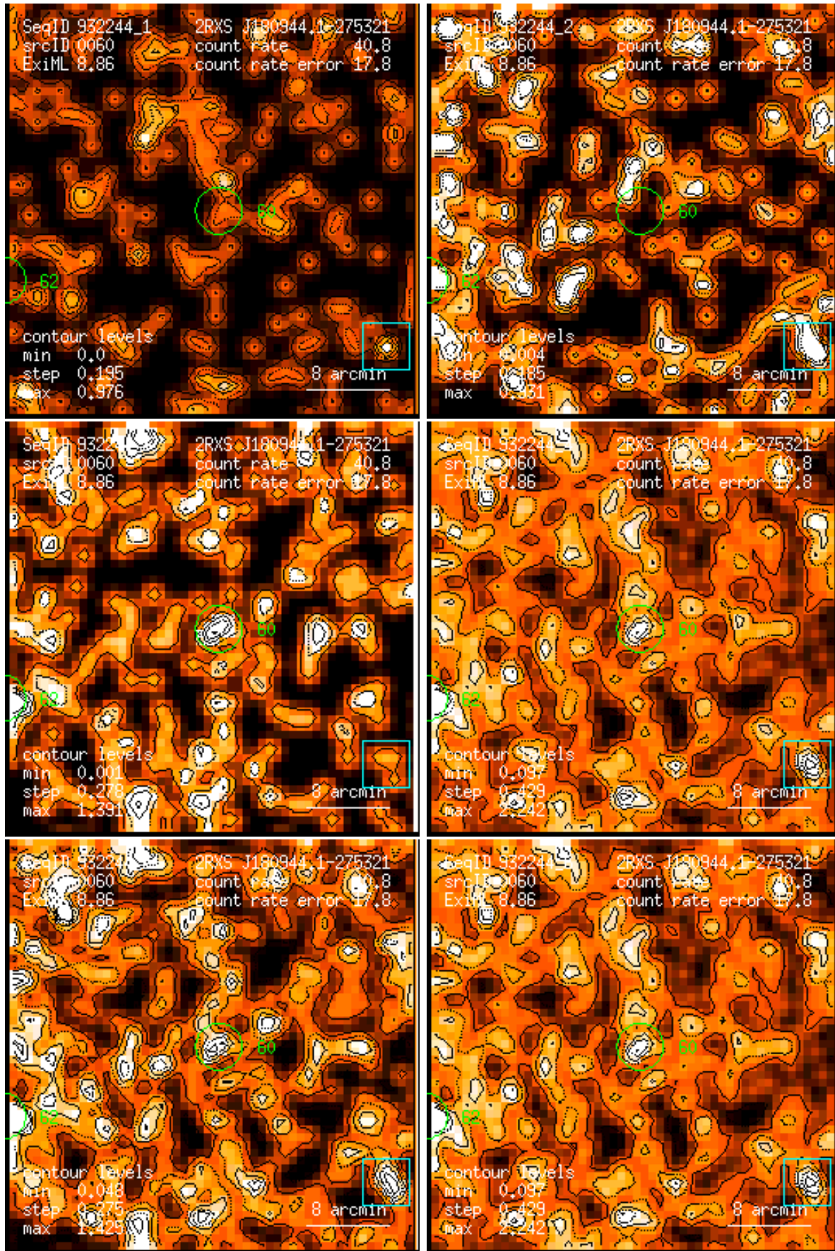
Figure 60: RASS 932244: detection 0060: band rate images, Gaussian filter: (1) PSPC channels 11 – 41, (2) 52 – 90, (3) 91 – 201, (4) 11 – 235, (5) 52 – 201, (6) 11 – 201. Broad band rates in counts/ks. Band rate contour levels in counts/ks/arcmin 2 .
