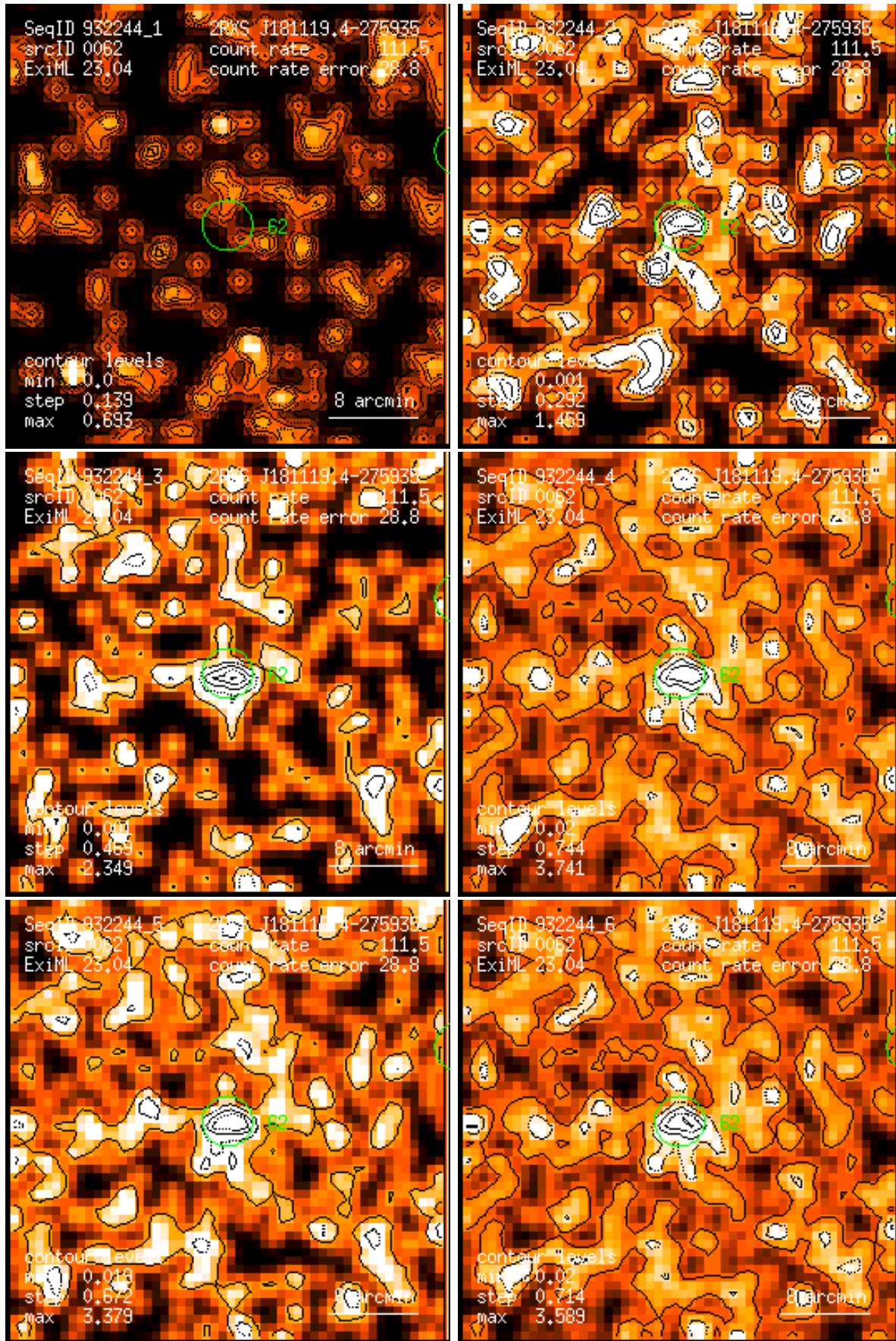
Figure 62: RASS 932244: detection 0062: band rate images, Gaussian filter: (1) PSPC channels 11 – 41, (2) 52 – 90, (3) 91 – 201, (4) 11 – 235, (5) 52 – 201, (6) 11 – 201. Broad band rates in counts/ks. Band rate contour levels in counts/ks/arcmin 2 .
