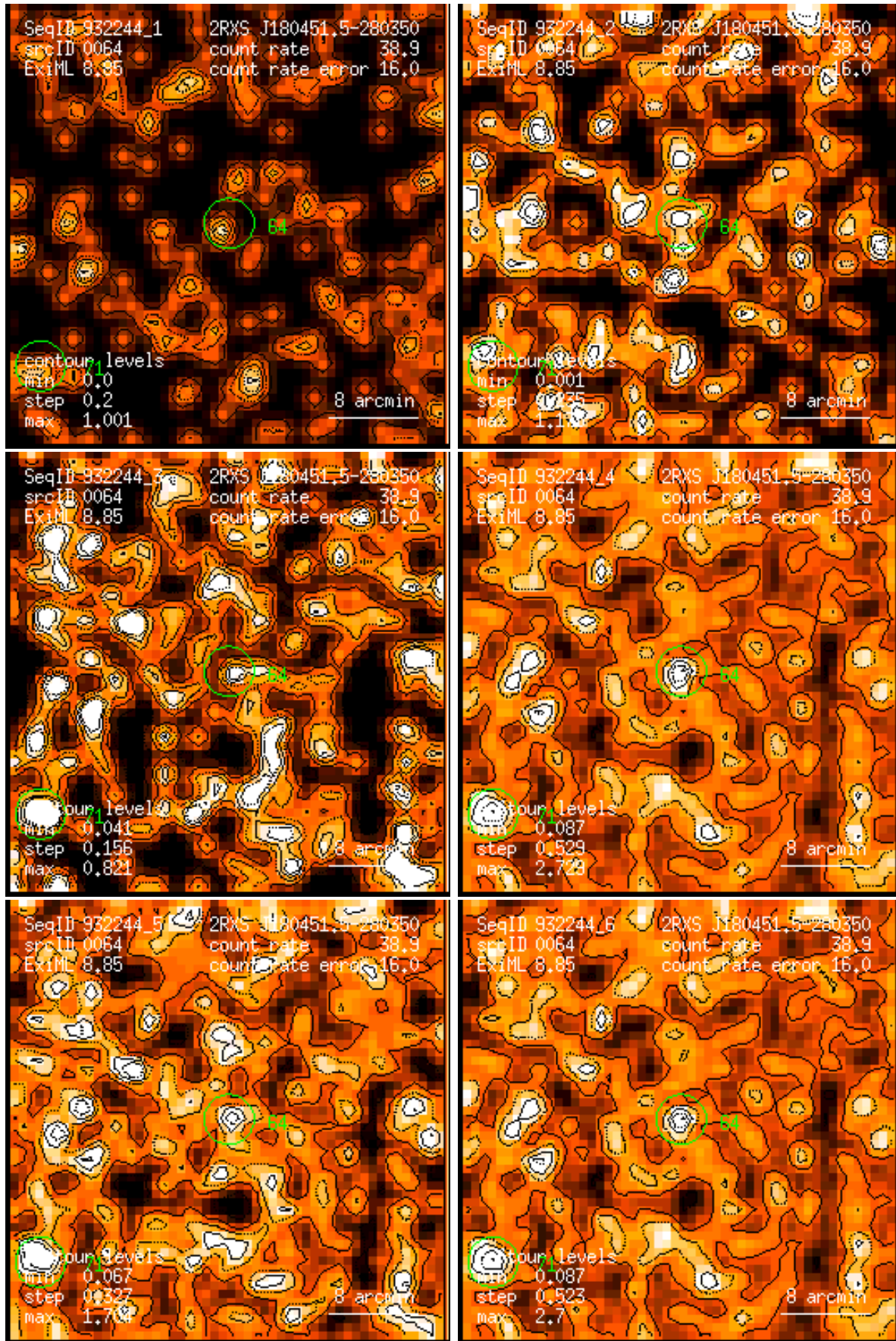
Figure 64: RASS 932244: detection 0064: band rate images, Gaussian filter: (1) PSPC channels 11 – 41, (2) 52 – 90, (3) 91 – 201, (4) 11 – 235, (5) 52 – 201, (6) 11 – 201. Broad band rates in counts/ks. Band rate contour levels in counts/ks/arcmin 2 .
