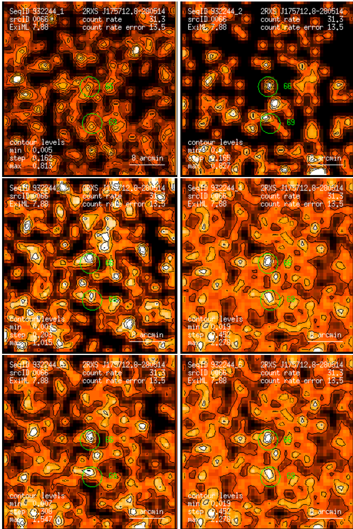
Figure 66: RASS 932244: detection 0066: band rate images, Gaussian filter: (1) PSPC channels 11 – 41, (2) 52 – 90, (3) 91 – 201, (4) 11 – 235, (5) 52 – 201, (6) 11 – 201. Broad band rates in counts/ks. Band rate contour levels in counts/ks/arcmin 2 .
